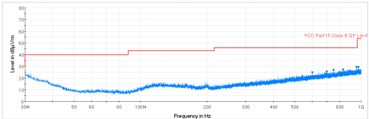
Plot 7-54. Radiated Spurious Plot below 1GHz (Pol. V)
