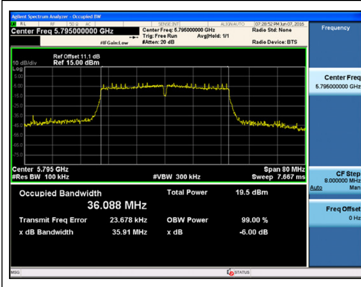
802.11n_HT40 UNII 3 BAND 6dB Bandwidth(CH.159)
