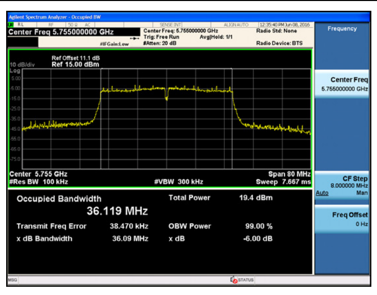
802.11ac_VHT40 UNII 3 BAND 6dB Bandwidth(CH.151)
