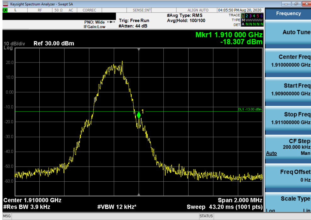
Plot 7-77. Band Edge Plot (PCS GSM Mode - High Channel)
