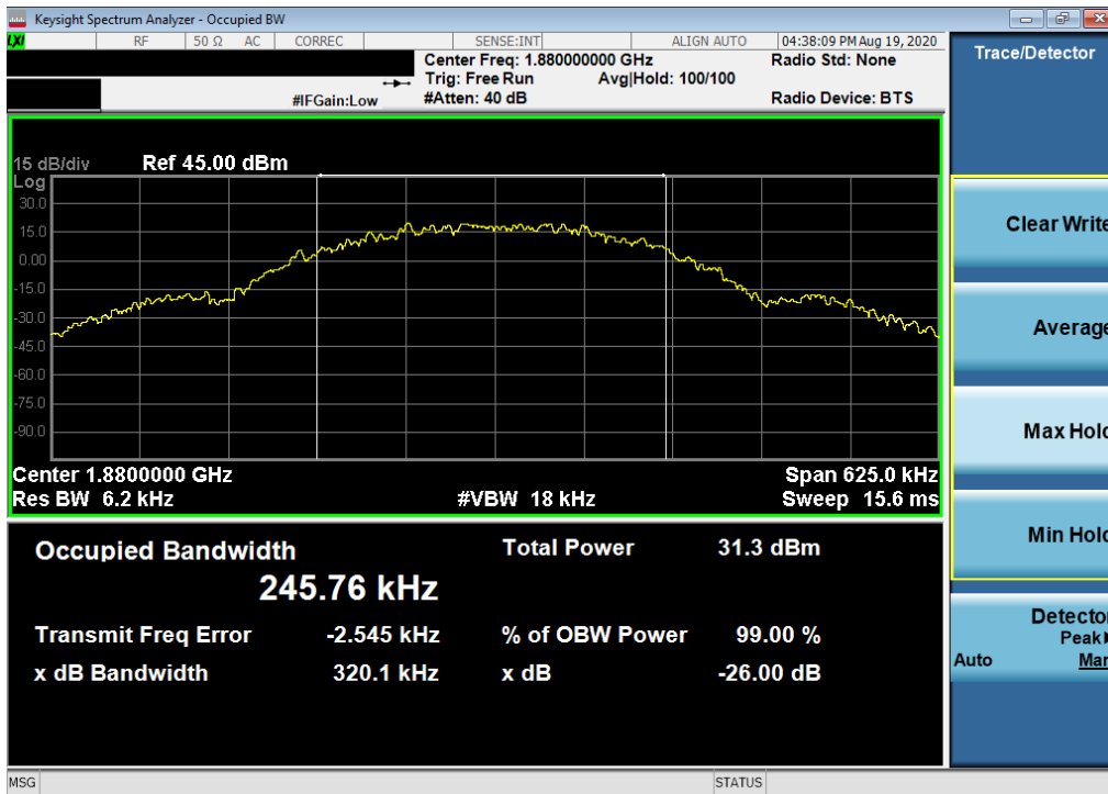
Plot 7-2. Occupied Bandwidth Plot (PCS GPRS Mode)
