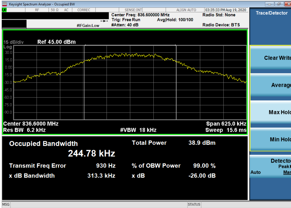
Plot 7-1. Occupied Bandwidth Plot (Cellular GPRS Mode)
