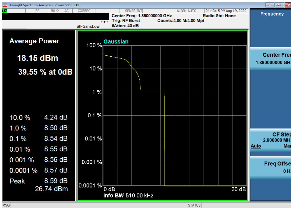
Plot 7-100. Peak-Average Ratio Plot (EDGE1900 Mode)
