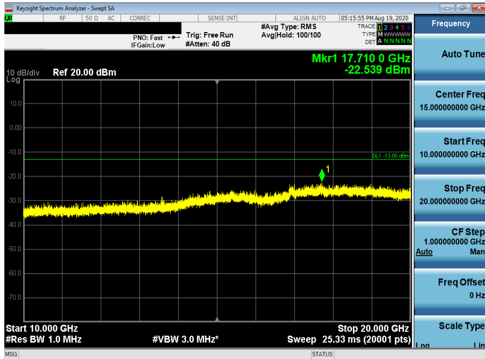
Plot 7-24. Conducted Spurious Plot (PCS GSM Mode - Mid Channel)
