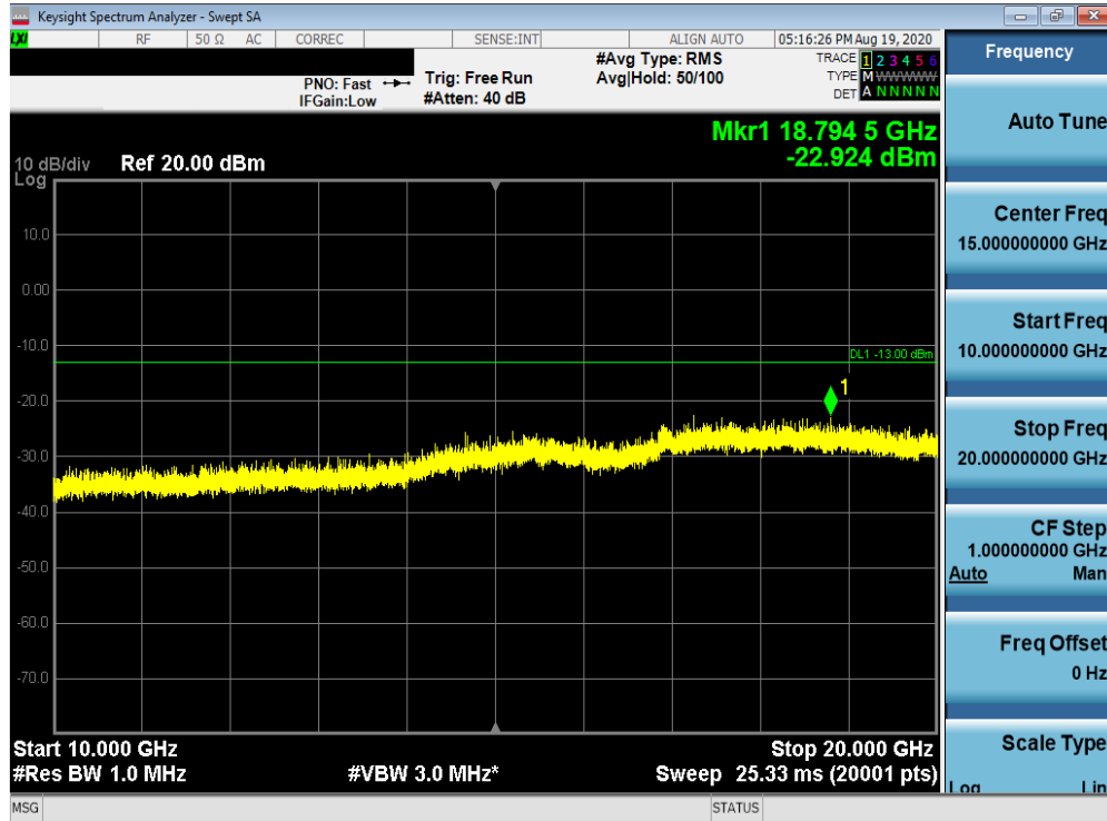
Plot 7-21. Conducted Spurious Plot (PCS GSM Mode - Low Channel)
