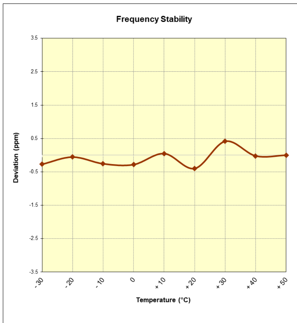
Figure 7-9. Frequency Stability Graph (Cellular GSM Mode – Ch. 190)
