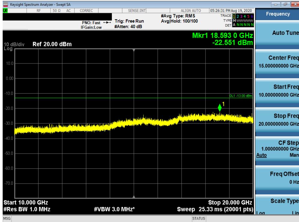
Plot 7-27. Conducted Spurious Plot (PCS GSM Mode - High Channel)
