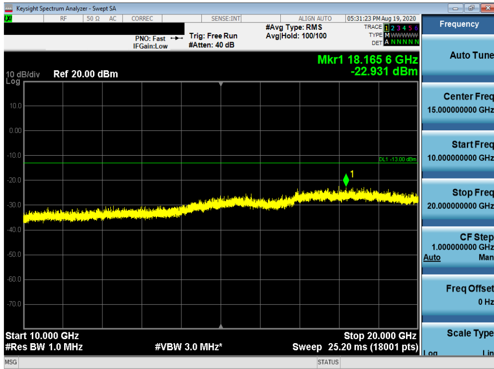
Plot 7-12. Conducted Spurious Plot (Cellular GSM Mode - Low Channel)
