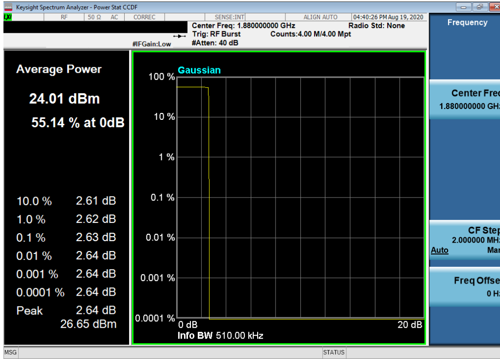
Plot 7-99. Peak-Average Ratio Plot (PCS GSM Mode)
