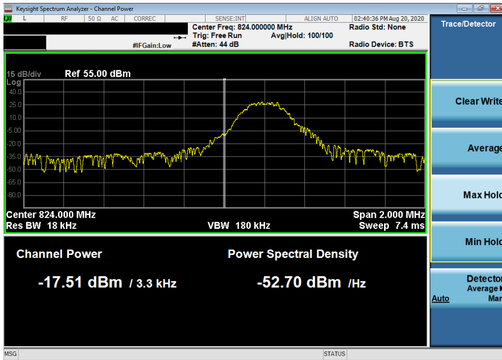
Plot 7-73. Band Edge Plot (Cellular GSM Mode - Low Channel)
