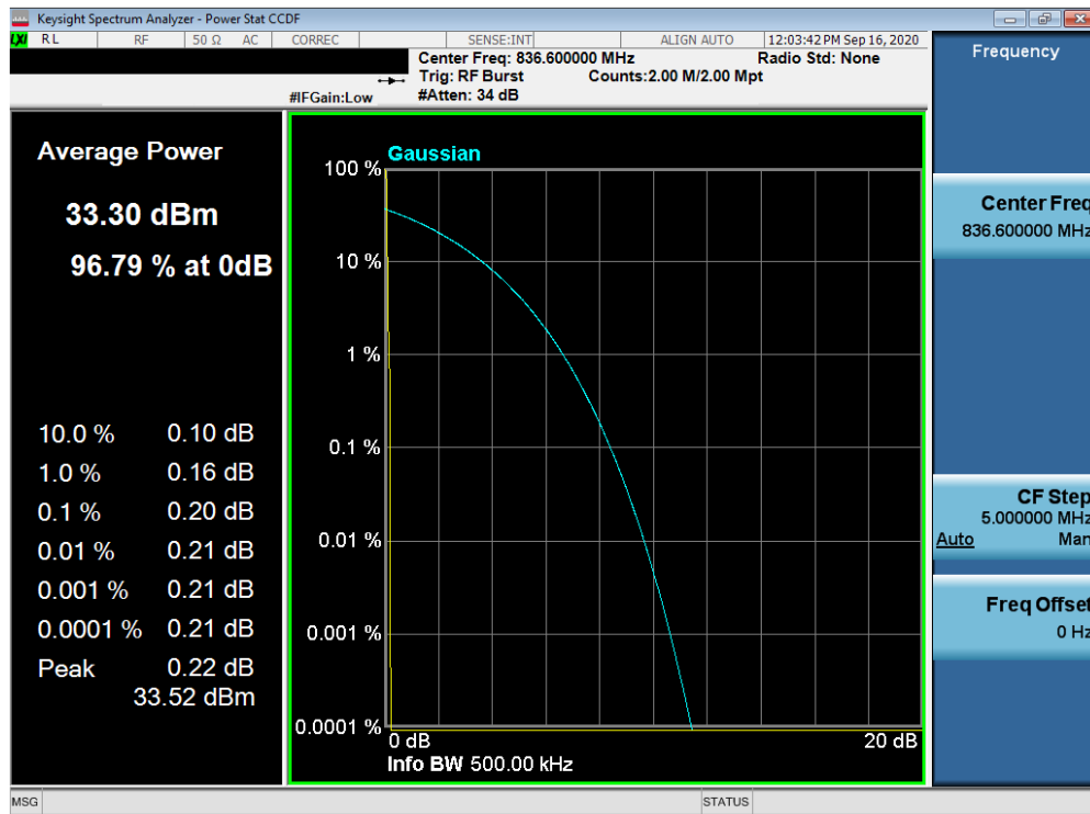
Plot 7-97. Peak-Average Ratio Plot (Cellular GSM Mode)
