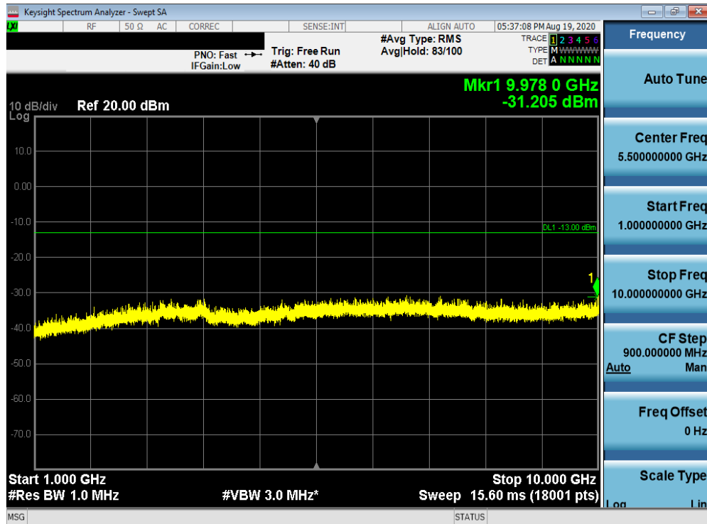
Plot 7-15. Conducted Spurious Plot (Cellular GSM Mode - Mid Channel)
