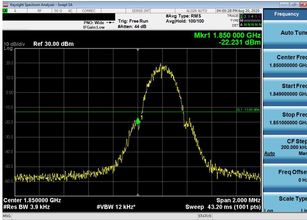
Plot 7-75. Band Edge Plot (PCS GSM Mode - Low Channel)
