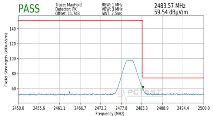
Plot 7-52. Radiated Restricted Upper Band Edge Measurement (Peak)
