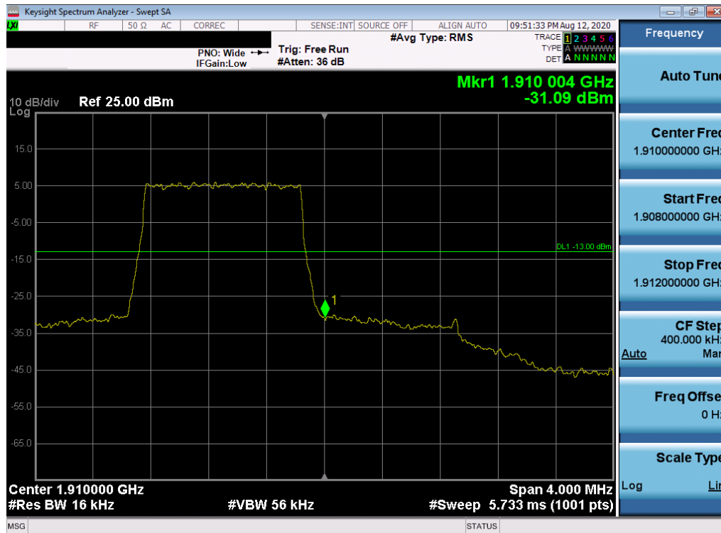
Plot 7-380. Upper Band Edge Plot (LTE Band 2 – 1.4MHz QPSK – Full RB Configuration)
