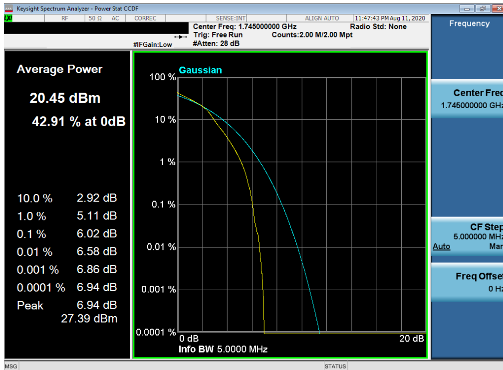
Plot 7-489. PAR Plot (LTE Band 66/4 - 5MHz 16-QAM - Full RB Configuration)
