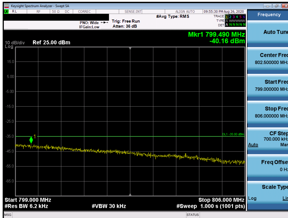
Plot 7-49. Emission Mask Plot (LTE Band 14 - 10MHz QPSK - High Channel)
