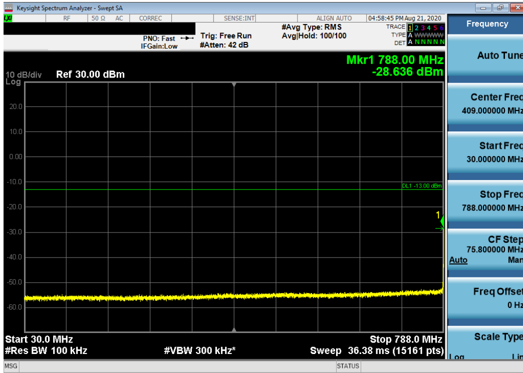
Plot 7-33. Conducted Spurious Plot (LTE Band 14 - 10MHz QPSK - RB Size 1, RB Offset 0)
