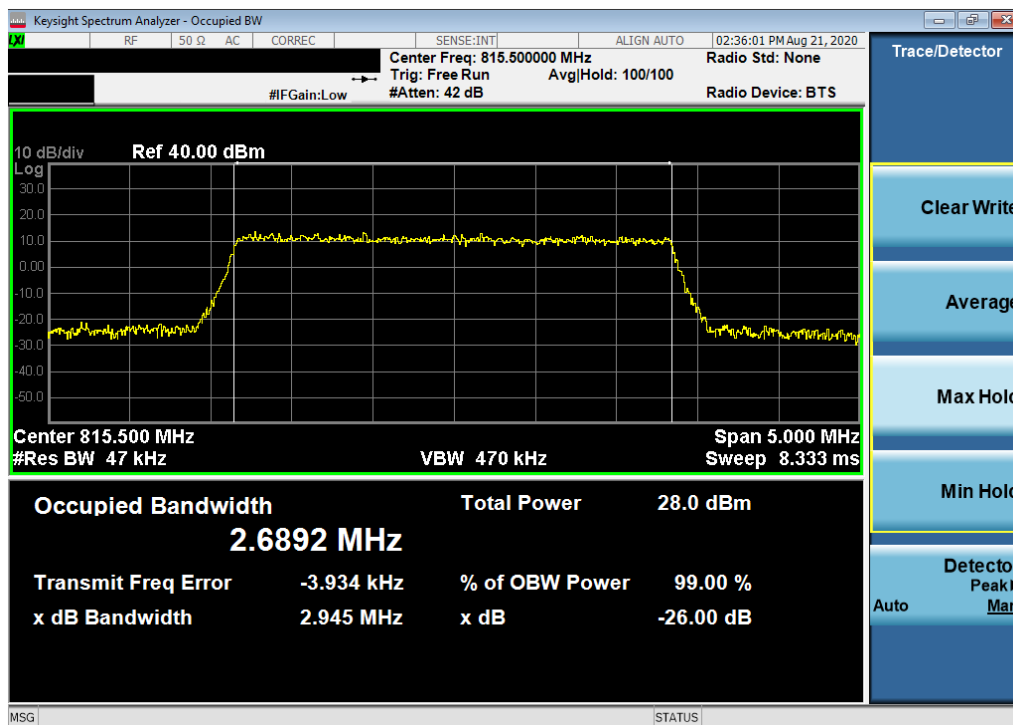
Plot 7-14. Occupied Bandwidth Plot (LTE Band 26 - 3MHz 64-QAM - Full RB Configuration)
