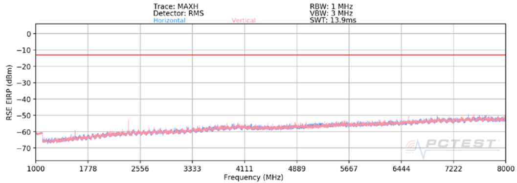
Plot 7-58. Radiated Spurious Plot (LTE Band 14)
