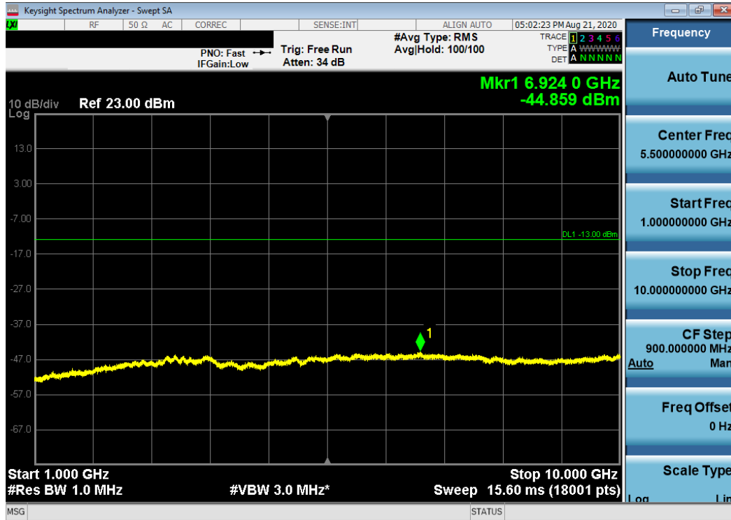
Plot 7-35. Conducted Spurious Plot (LTE Band 14 - 10MHz QPSK - RB Size 1, RB Offset 0)
