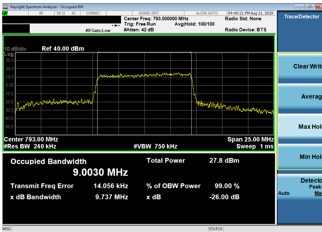
Plot 7-20. Occupied Bandwidth Plot (LTE Band 14 - 10MHz 64-QAM - Full RB Configuration)
