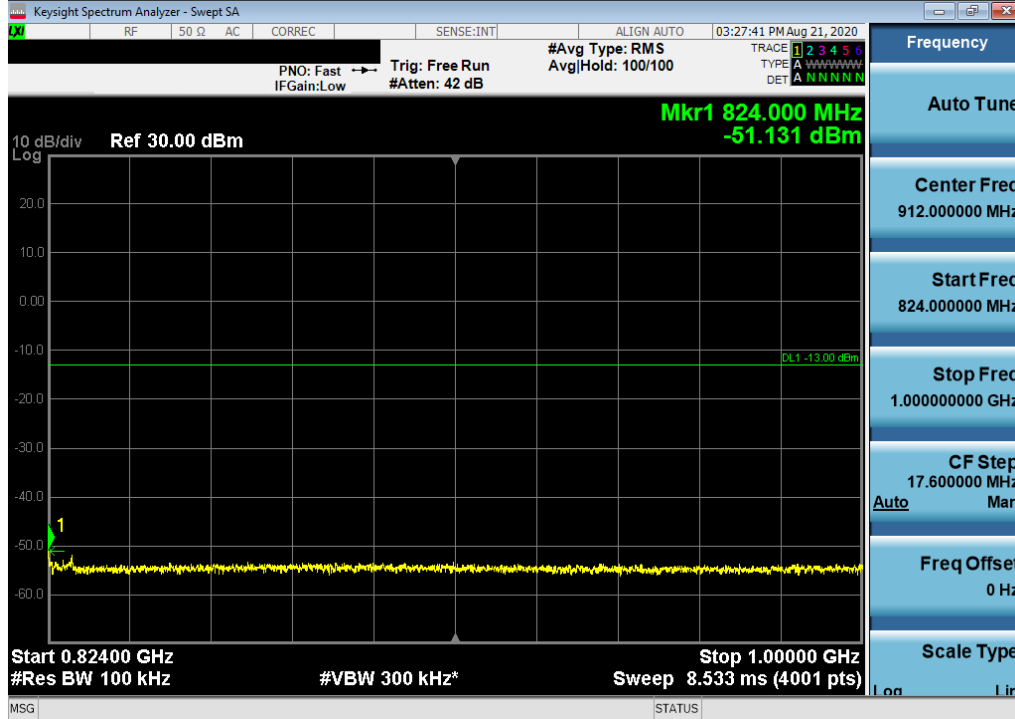
Plot 7-31. Conducted Spurious Plot (LTE Band 26 - 15MHz QPSK - RB Size 1, RB Offset 0)
