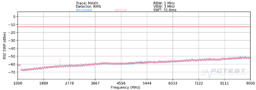
Plot 7-57. Radiated Spurious Plot (LTE Band 26)
