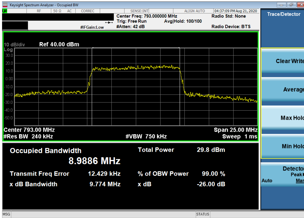
Plot 7-18. Occupied Bandwidth Plot (LTE Band 14 - 10MHz QPSK - Full RB Configuration)
