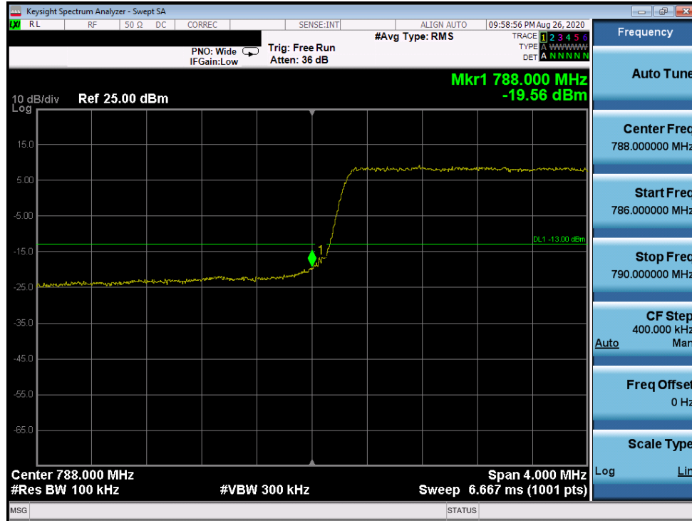
Plot 7-50. Band Edge Plot (LTE Band 14 - 5MHz QPSK - Low Channel)
