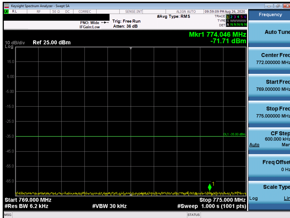
Plot 7-51. Emission Mask Plot (LTE Band 14 - 5MHz QPSK - Low Channel)
