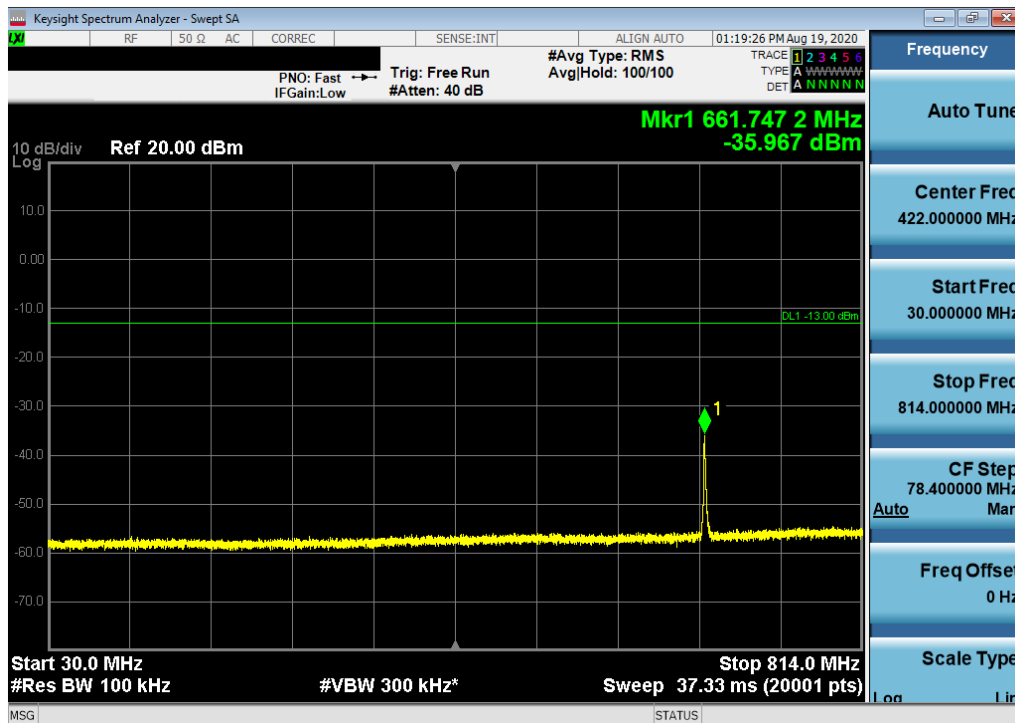
Plot 7-27. Conducted Spurious Plot (CDMA/EvDO, Ch. 684)
