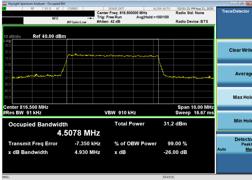
Plot 7-9. Occupied Bandwidth Plot (LTE Band 26 - 5MHz QPSK - Full RB Configuration)
