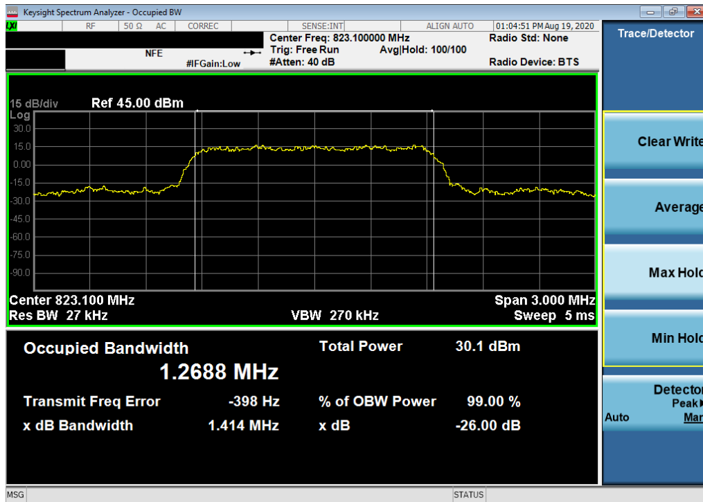
Plot 7-2. Occupied Bandwidth Plot (CDMA/EvDO, Ch. 684)
