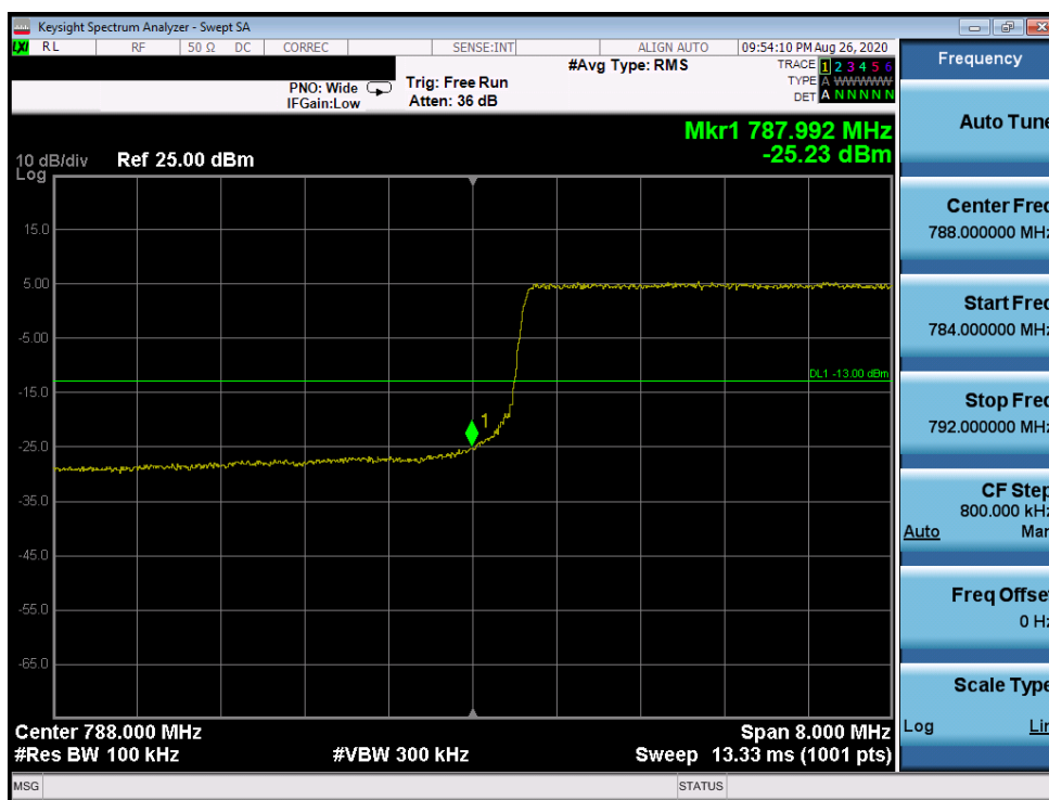
Plot 7-46. Band Edge Plot (LTE Band 14 - 10MHz QPSK - Low Channel)
