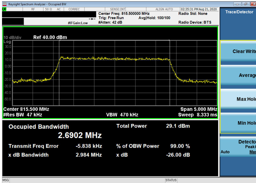
Plot 7-13. Occupied Bandwidth Plot (LTE Band 26 - 3MHz 16-QAM - Full RB Configuration)
