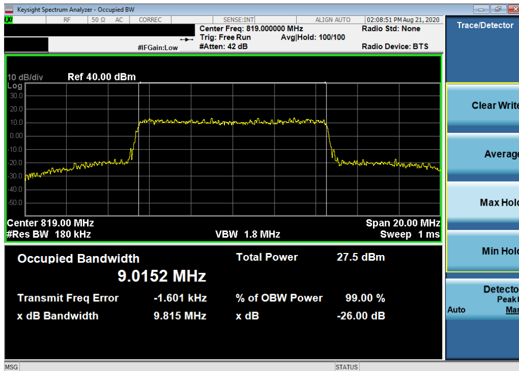
Plot 7-8. Occupied Bandwidth Plot (LTE Band 26 - 10MHz 64-QAM - Full RB Configuration)
