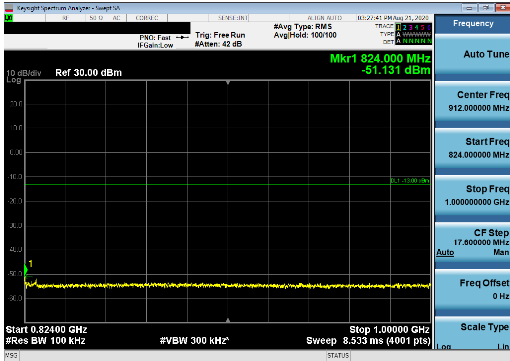
Plot 7-32. Conducted Spurious Plot (LTE Band 26 - 15MHz QPSK - RB Size 1, RB Offset 0)
