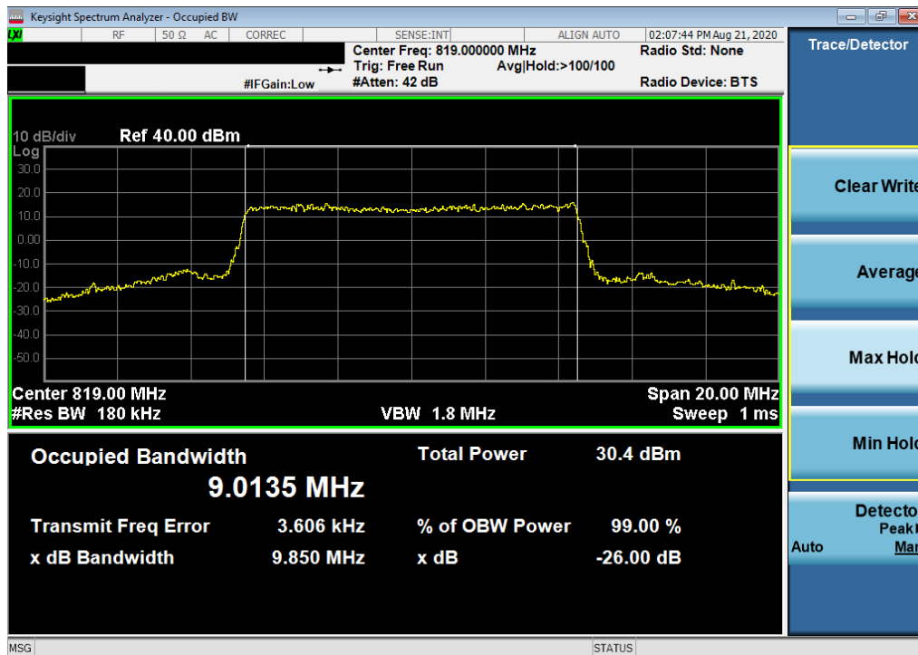
Plot 7-6. Occupied Bandwidth Plot (LTE Band 26 - 10MHz QPSK - Full RB Configuration)
