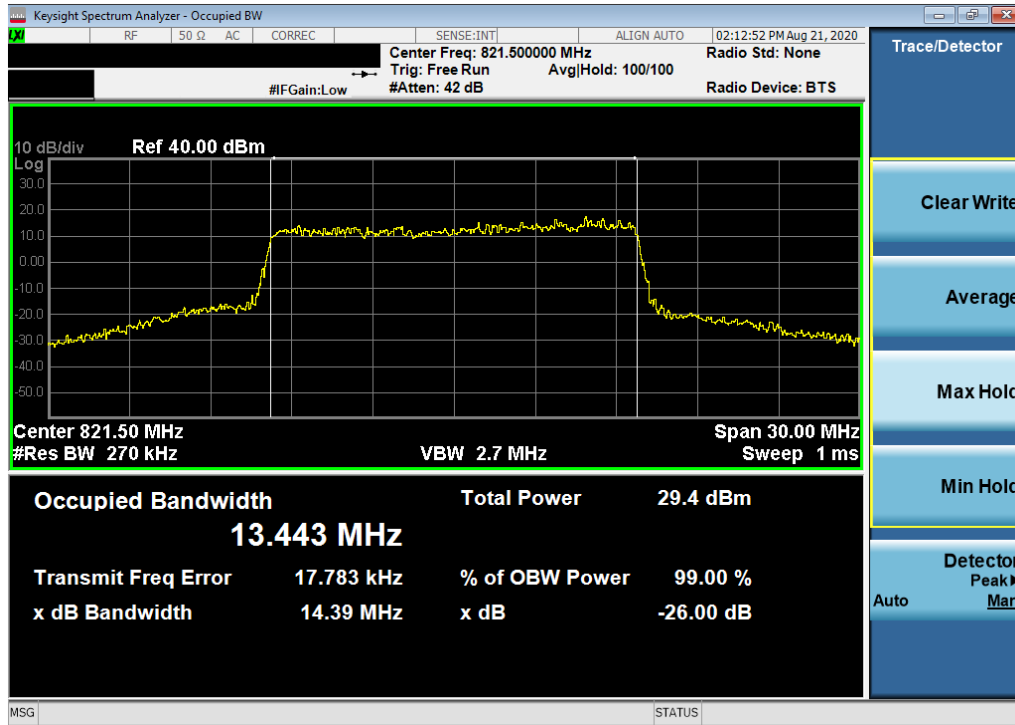
Plot 7-3. Occupied Bandwidth Plot (LTE Band 26 - 15MHz QPSK - Full RB Configuration)
