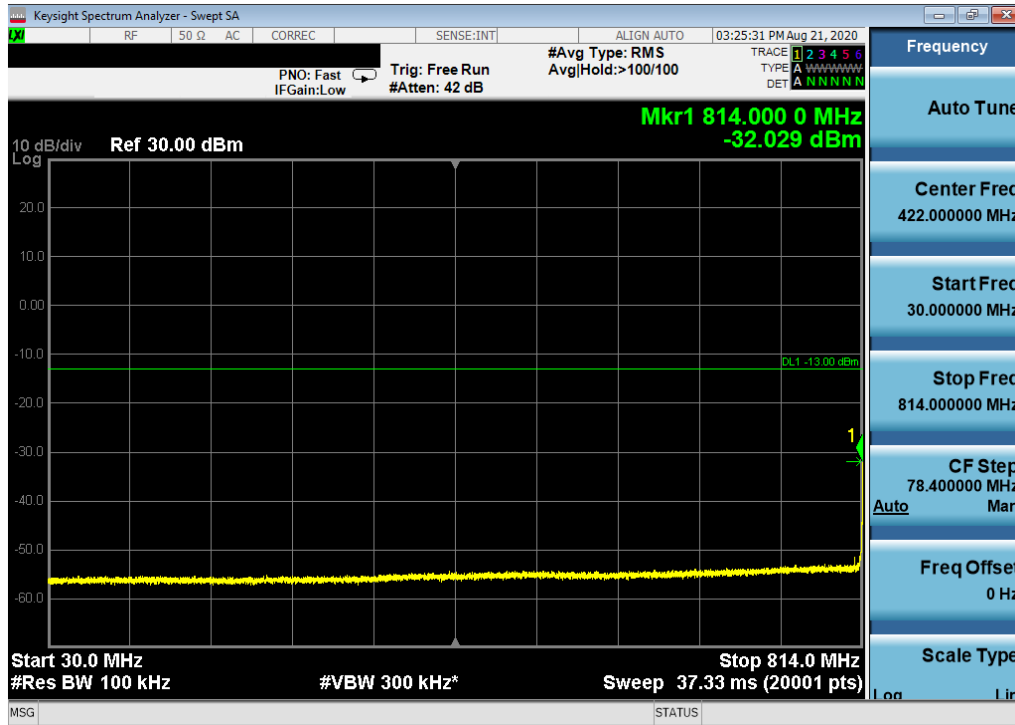
Plot 7-30. Conducted Spurious Plot (LTE Band 26 - 15MHz QPSK - RB Size 1, RB Offset 0)
