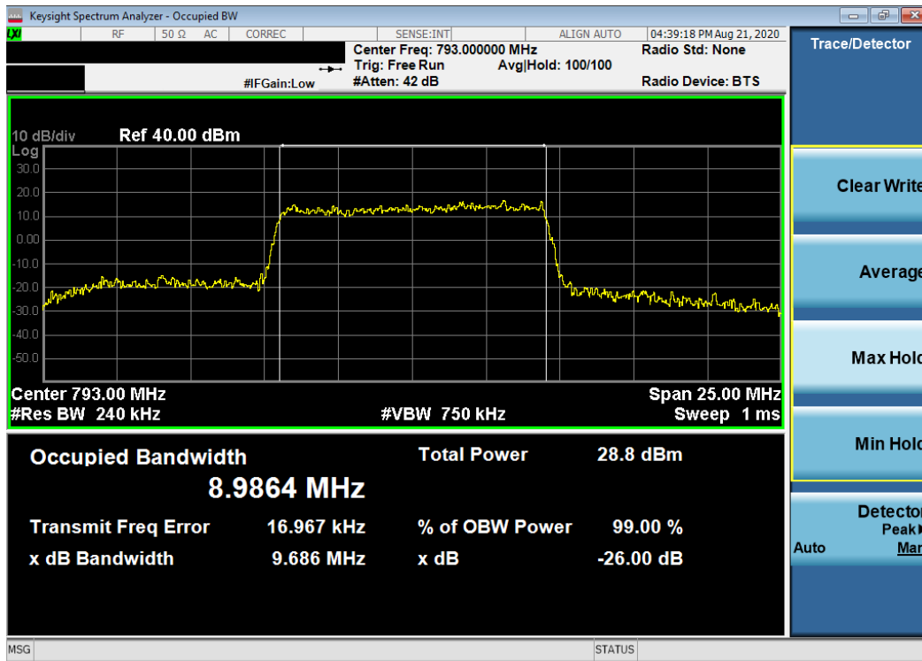
Plot 7-19. Occupied Bandwidth Plot (LTE Band 14 - 10MHz 16-QAM - Full RB Configuration)
