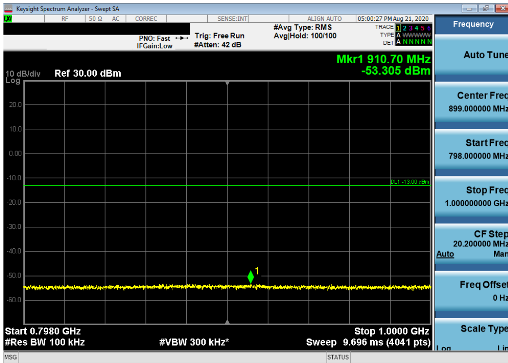
Plot 7-34. Conducted Spurious Plot (LTE Band 14 - 10MHz QPSK - RB Size 1, RB Offset 0)
