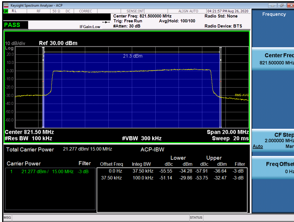
Plot 7-38. Channel Edge Plot (LTE Band 26 - 15MHz QPSK)
