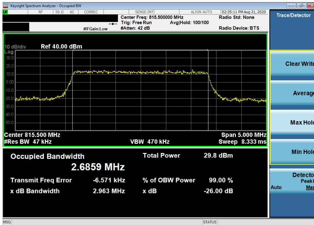
Plot 7-12. Occupied Bandwidth Plot (LTE Band 26 - 3MHz QPSK - Full RB Configuration)
