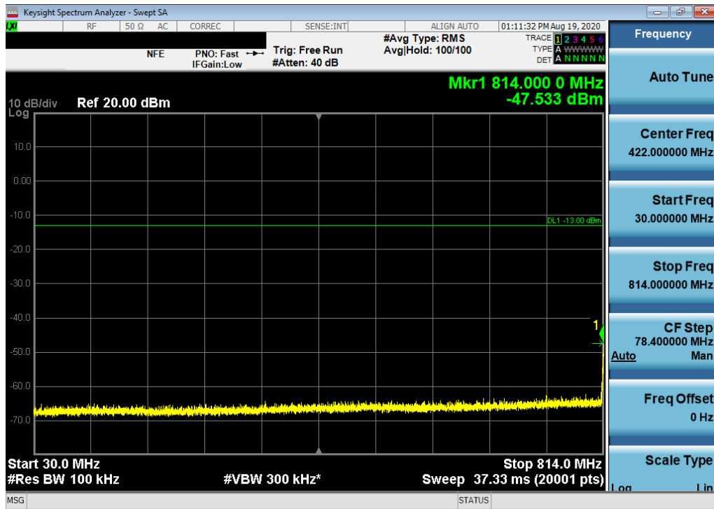
Plot 7-24. Conducted Spurious Plot (CDMA/EvDO, Ch. 476)
