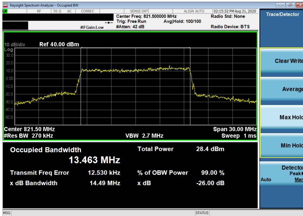
Plot 7-4. Occupied Bandwidth Plot (LTE Band 26 - 15MHz 16-QAM - Full RB Configuration)
