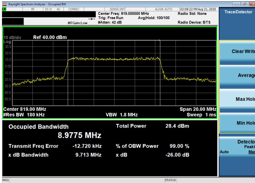
Plot 7-7. Occupied Bandwidth Plot (LTE Band 26 - 10MHz 16-QAM - Full RB Configuration)
