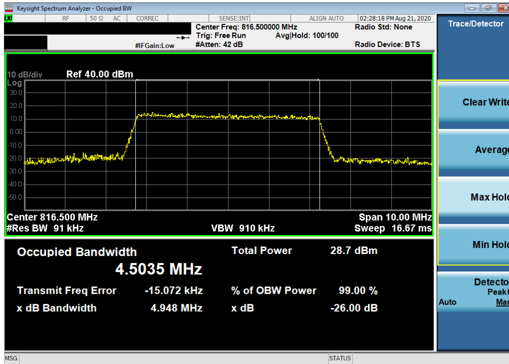
Plot 7-11. Occupied Bandwidth Plot (LTE Band 26 - 5MHz 64-QAM - Full RB Configuration)
