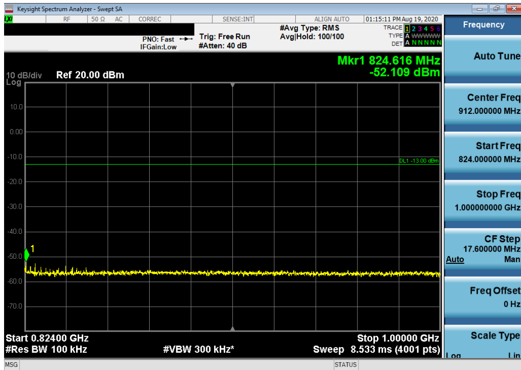
Plot 7-25. Conducted Spurious Plot (CDMA/EvDO, Ch. 476)
