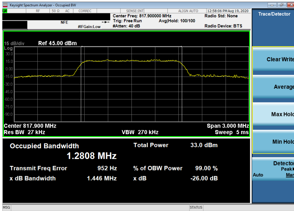
Plot 7-1. Occupied Bandwidth Plot (CDMA/EvDO, Ch. 476)
