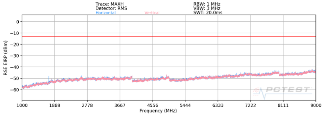
Plot 7-56. CDMA BC10 Radiated Spurious Plot
