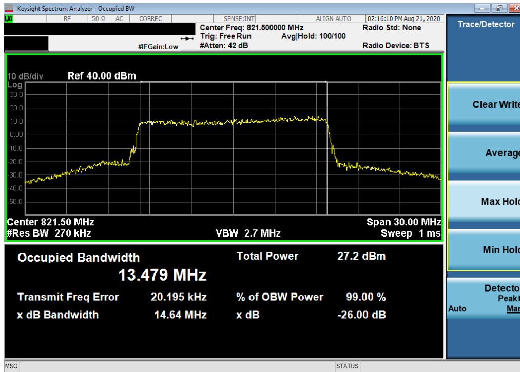
Plot 7-5. Occupied Bandwidth Plot (LTE Band 26 - 15MHz 64-QAM - Full RB Configuration)
