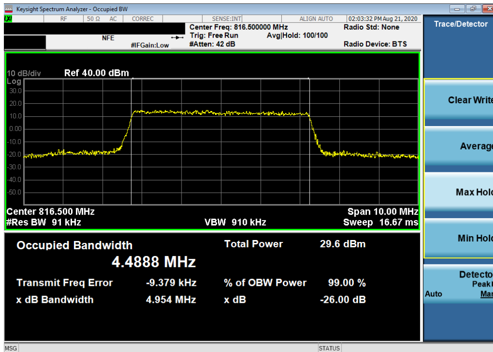
Plot 7-10. Occupied Bandwidth Plot (LTE Band 26 - 5MHz 16-QAM - Full RB Configuration)
