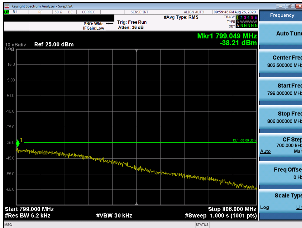
Plot 7-53. Emission Mask Plot (LTE Band 14 - 5MHz QPSK - High Channel)
