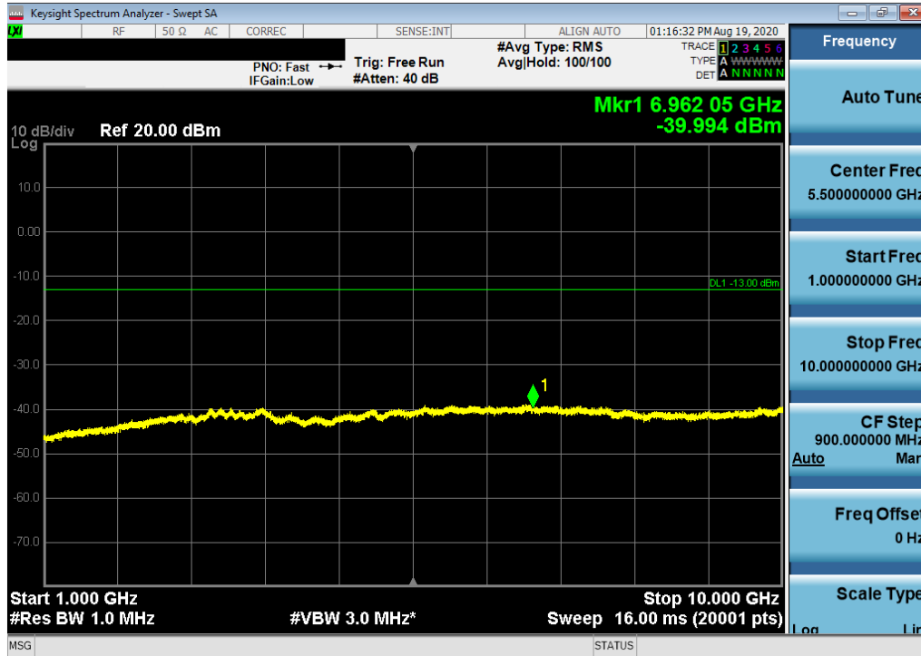
Plot 7-26. Conducted Spurious Plot (CDMA/EvDO, Ch. 476)
