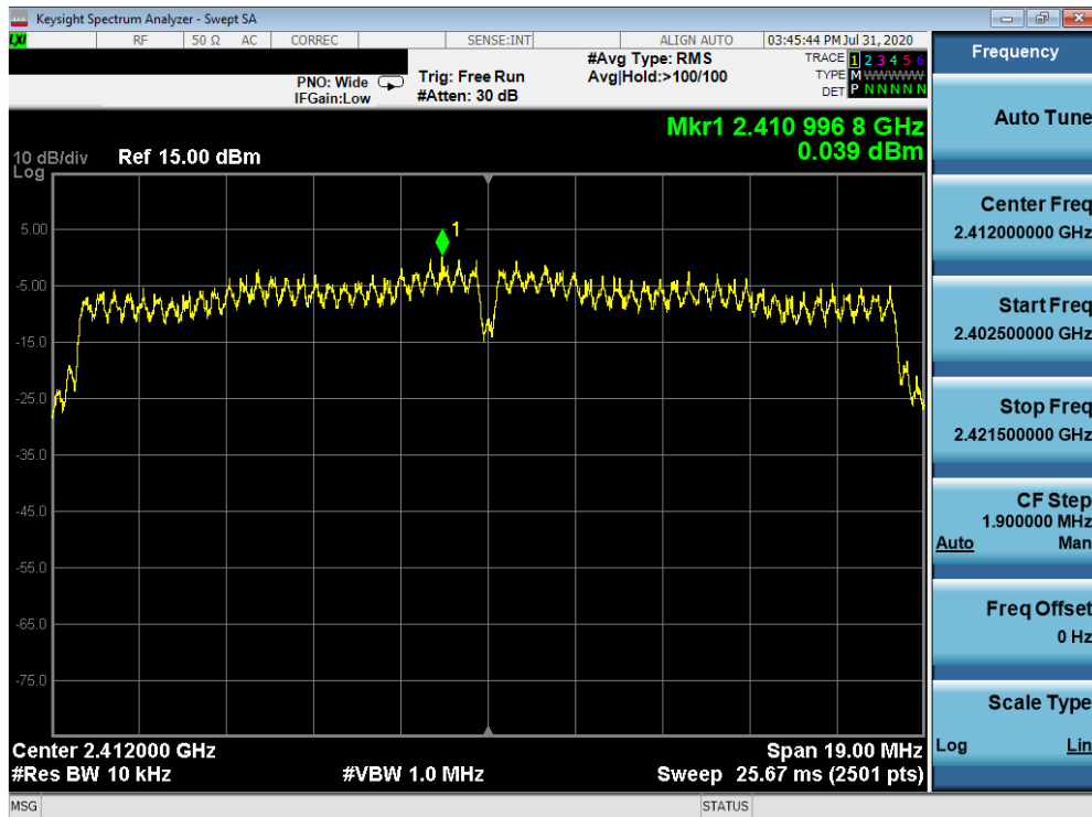
Plot 7-34. Power Spectral Density Plot SISO ANT1 (802.11ac (2.4GHz) – Ch. 1)
