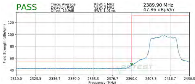
Plot 7-97. Radiated Restricted Lower Band Edge Measurement SISO ANT2 (Average)
