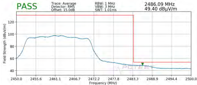
Plot 7-103. Radiated Restricted Upper Band Edge Measurement SISO ANT2 (Average)
