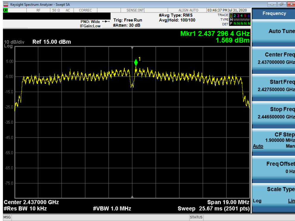
Plot 7-35. Power Spectral Density Plot SISO ANT1 (802.11ac (2.4GHz) – Ch. 6)
