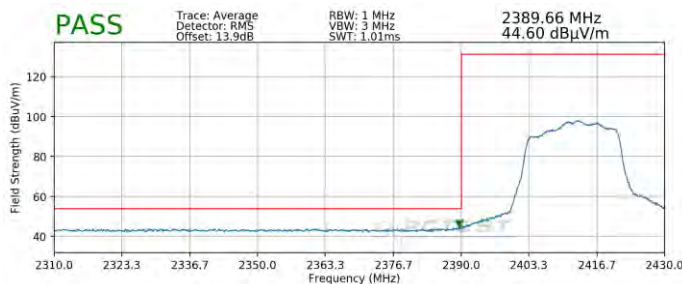
Plot 7-105. Radiated Restricted Lower Band Edge Measurement MIMO (Average)
