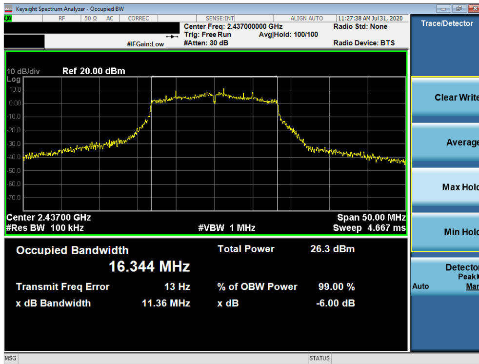
Plot 7-5. 6dB Bandwidth Plot SISO ANT1 (802.11g – Ch. 6)
