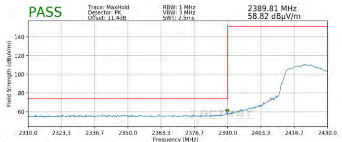
Plot 7-92. Radiated Restricted Lower Band Edge Measurement SISO ANT1 (Peak)
