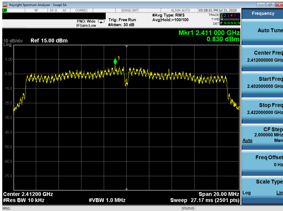
Plot 7-46. Power Spectral Density Plot SISO ANT1 (802.11ac (2.4GHz) – Ch. 1)
