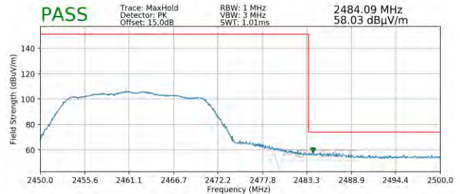
Plot 7-104. Radiated Restricted Upper Band Edge Measurement SISO ANT2 (Peak)
