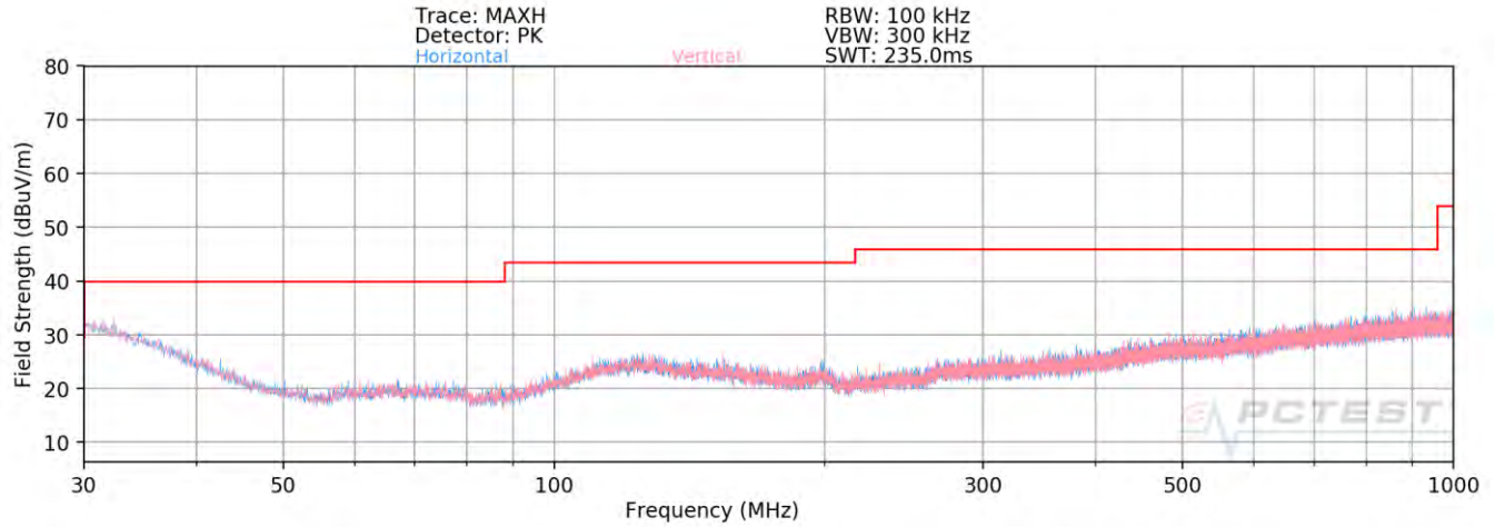
Plot 7-113. Radiated Spurious Plot below 1GHz MIMO
