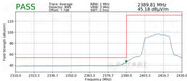
Plot 7-89. Radiated Restricted Lower Band Edge Measurement SISO ANT1 (Average)
