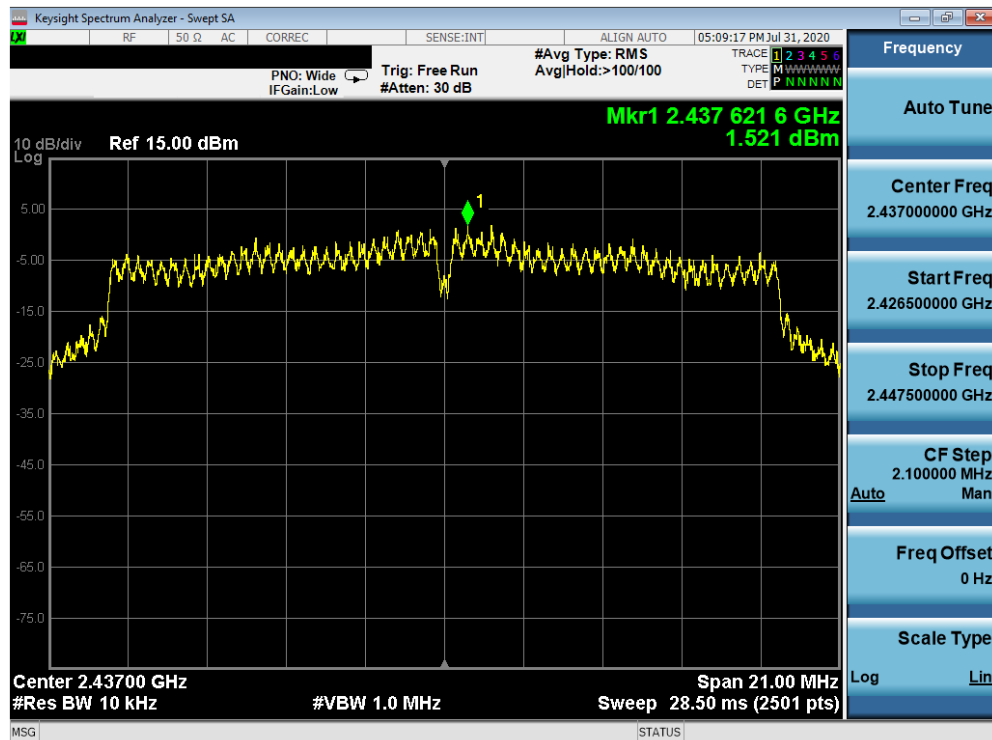
Plot 7-47. Power Spectral Density Plot SISO ANT1 (802.11ac (2.4GHz) – Ch. 6)
