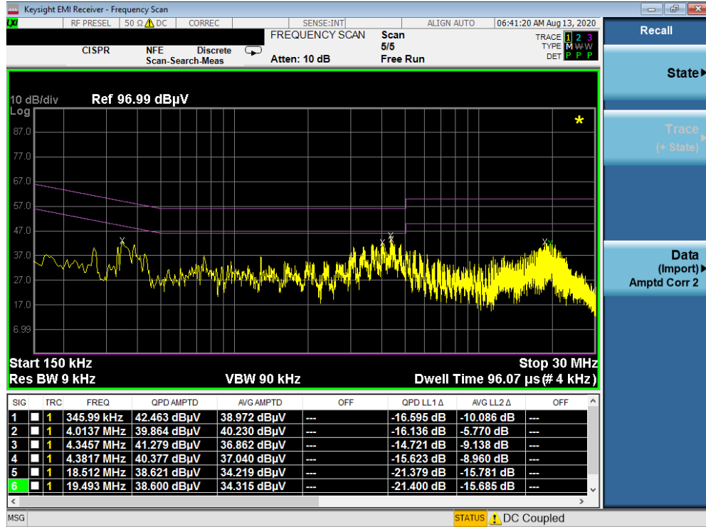
Plot 7-114. Line Conducted Plot with 802.11b (L1)
