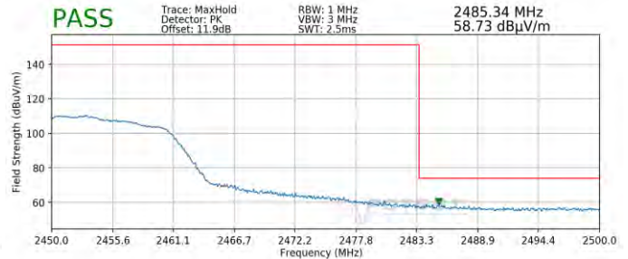
Plot 7-94. Radiated Restricted Upper Band Edge Measurement SISO ANT1 (Peak)
