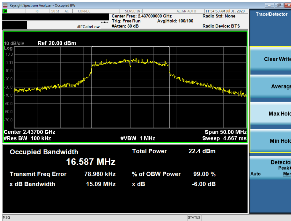
Plot 7-17. 6dB Bandwidth Plot SISO ANT2 (802.11g – Ch. 6)
