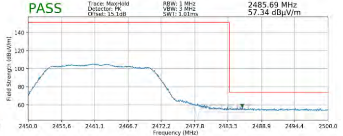
Plot 7-112. Radiated Restricted Upper Band Edge Measurement MIMO (Peak)
