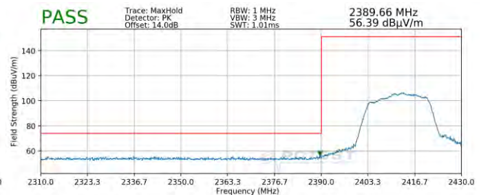
Plot 7-106. Radiated Restricted Lower Band Edge Measurement MIMO (Peak)
