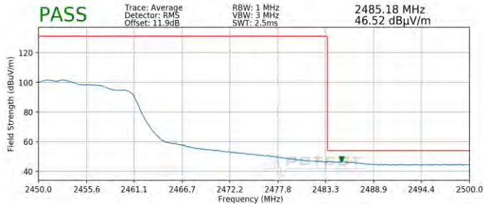
Plot 7-93. Radiated Restricted Upper Band Edge Measurement SISO ANT1 (Average)
