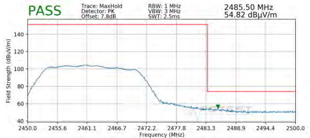
Plot 7-96. Radiated Restricted Upper Band Edge Measurement SISO ANT1 (Peak)
