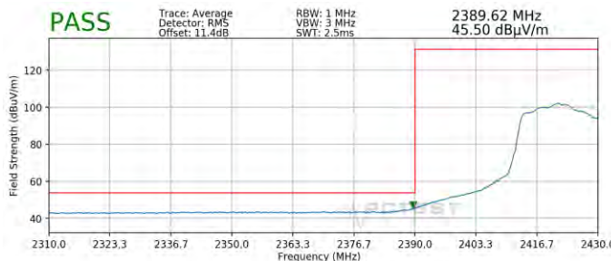
Plot 7-91. Radiated Restricted Lower Band Edge Measurement SISO ANT1 (Average)
