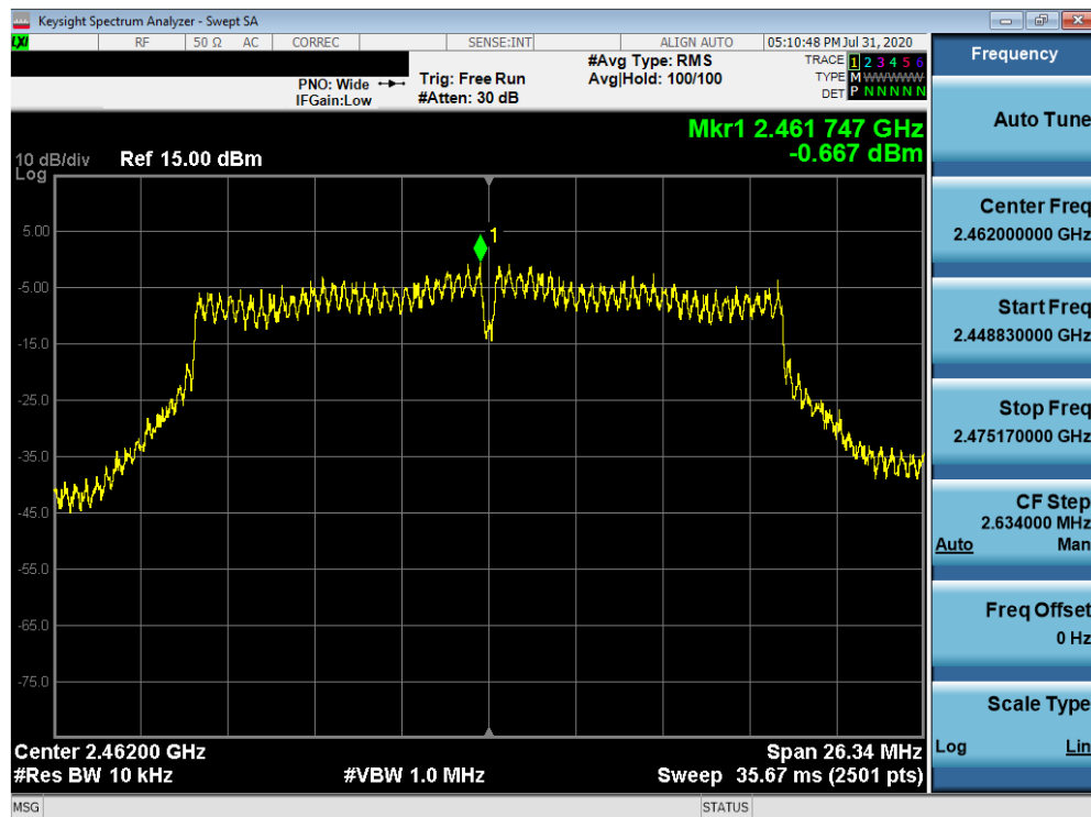
Plot 7-48. Power Spectral Density Plot SISO ANT1 (802.11ac (2.4GHz) – Ch. 11)
