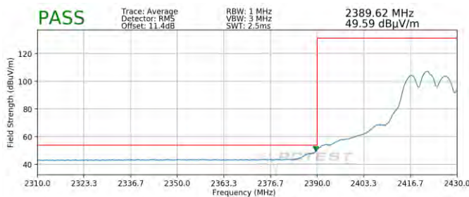
Plot 7-107. Radiated Restricted Lower Band Edge Measurement SISO ANT1 (Average)
