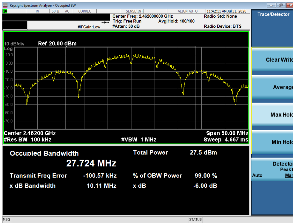
Plot 7-15. 6dB Bandwidth Plot SISO ANT2 (802.11b – Ch. 11)
