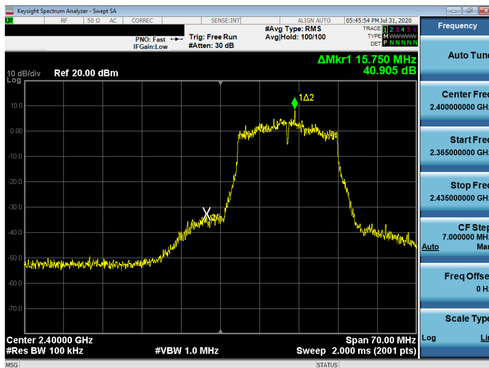
Plot 7-55. Band Edge Plot SISO ANT1 (802.11ac (2.4GHz) – Ch. 1)
