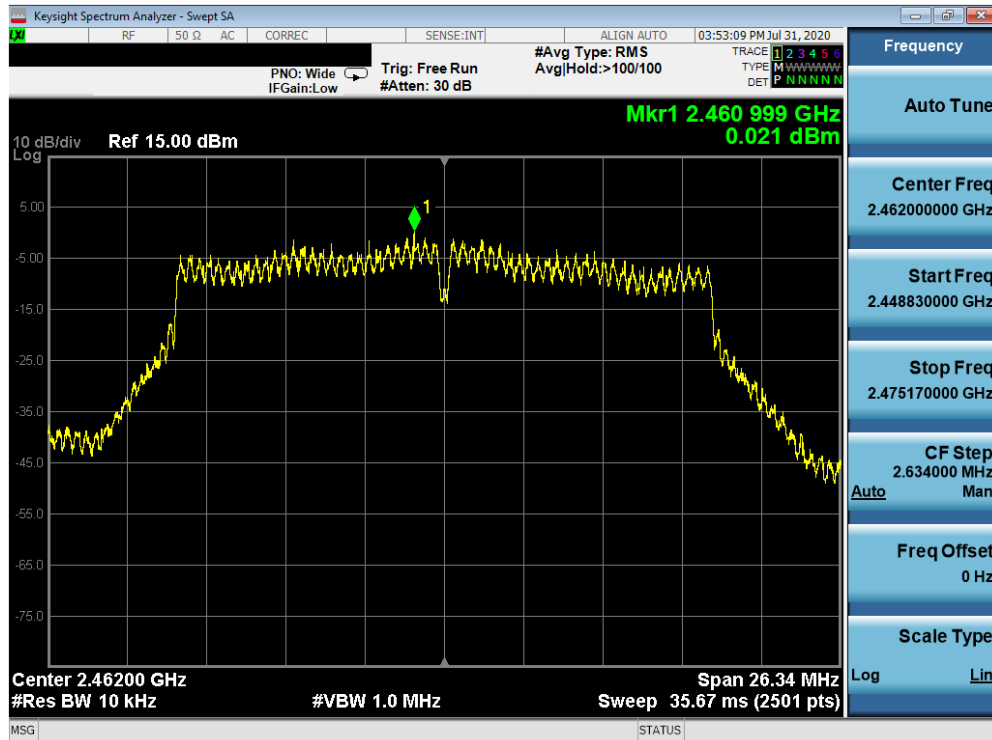
Plot 7-36. Power Spectral Density Plot SISO ANT1 (802.11ac (2.4GHz) – Ch. 11)
