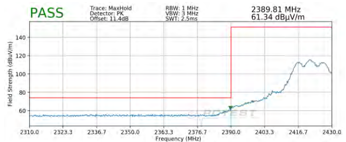
Plot 7-108. Radiated Restricted Lower Band Edge Measurement SISO ANT1 (Peak)
