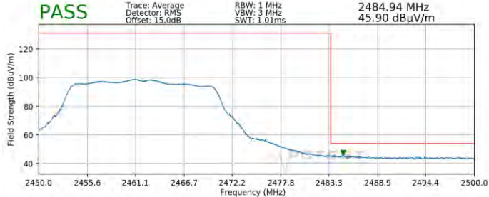
Plot 7-111. Radiated Restricted Upper Band Edge Measurement MIMO (Average)
