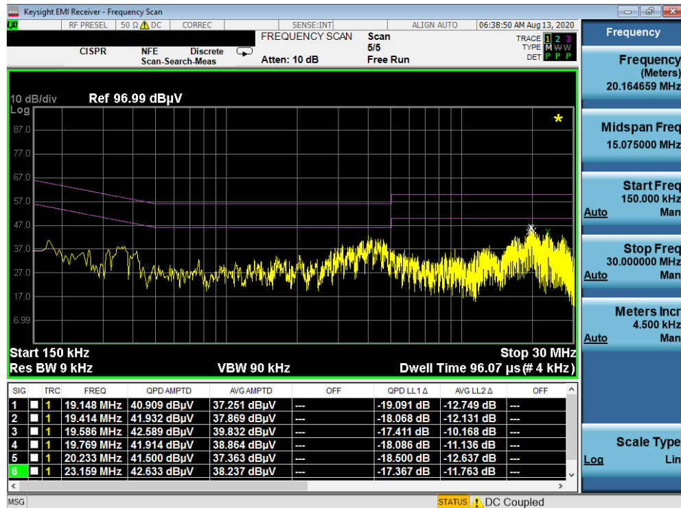
Plot 7-115. Line Conducted Plot with 802.11b (N)
