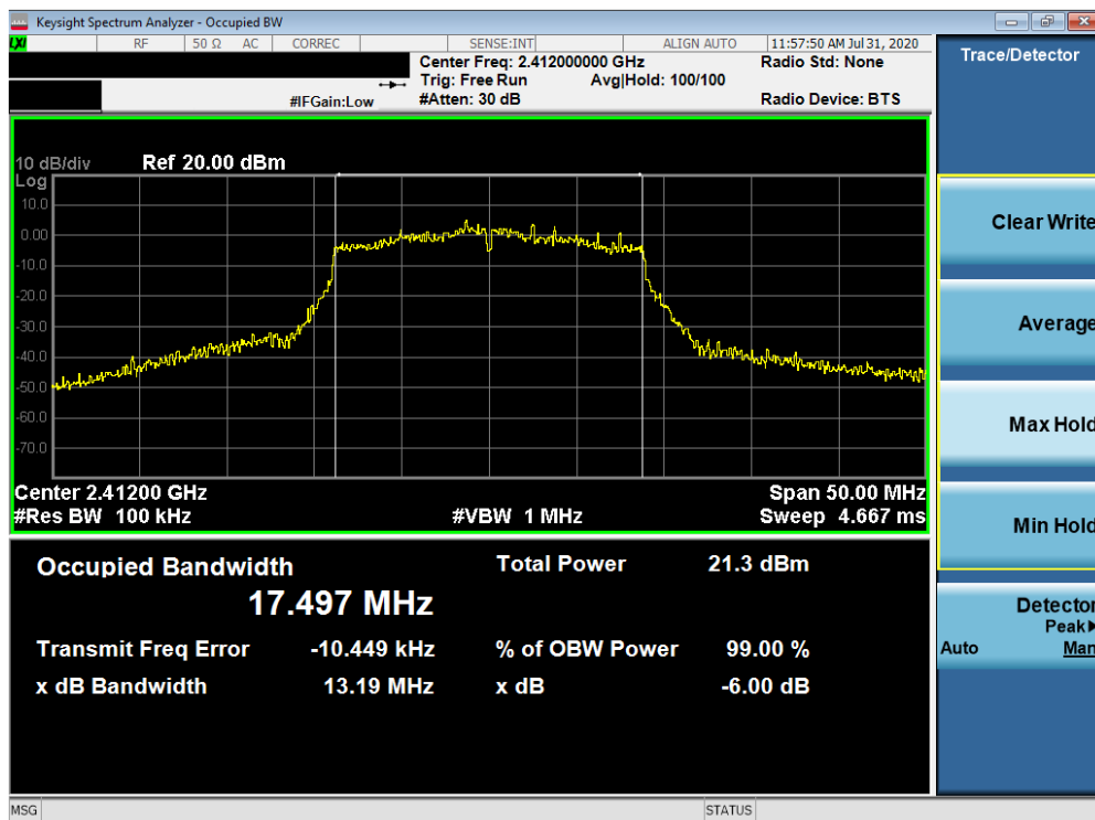
Plot 7-22. 6dB Bandwidth Plot SISO ANT2 (802.11ac (2.4GHz) – Ch. 1)
