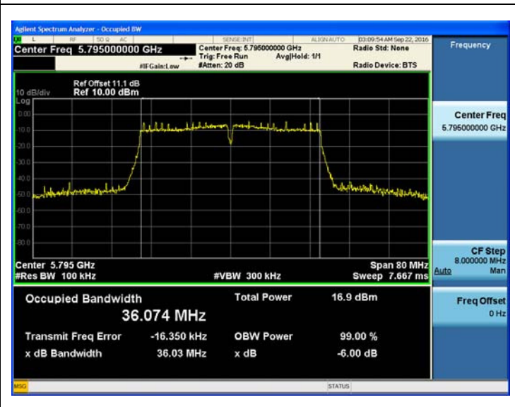
802.11ac_VHT40 UNII 3 BAND 6dB Bandwidth(CH.159)
