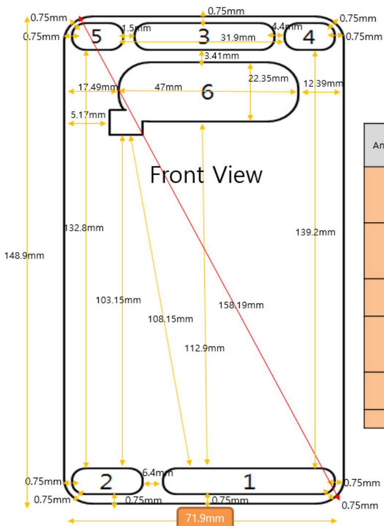
Antenna Distance
