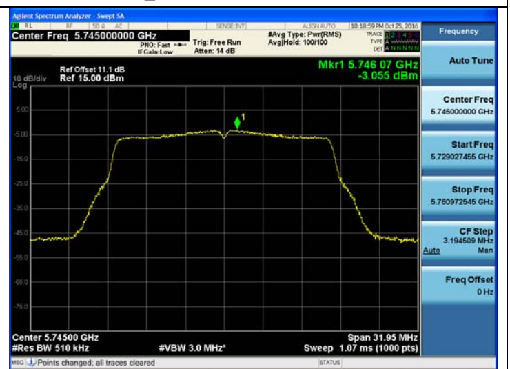
802.11ac_VHT20 UNII 3 BAND PSD CH 149
