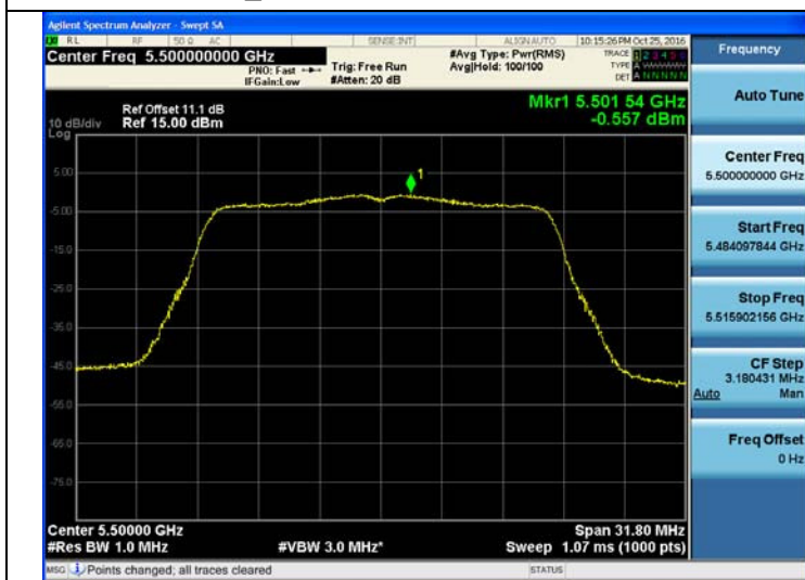
802.11ac_VHT20 UNII 2C BAND PSD CH 100
