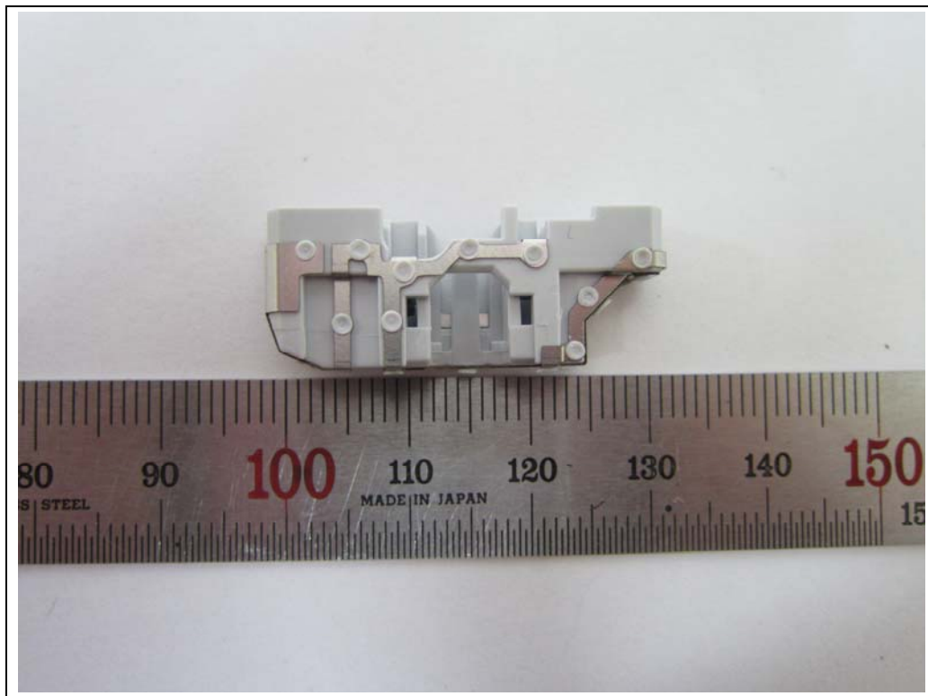
< Antenna 1 >
