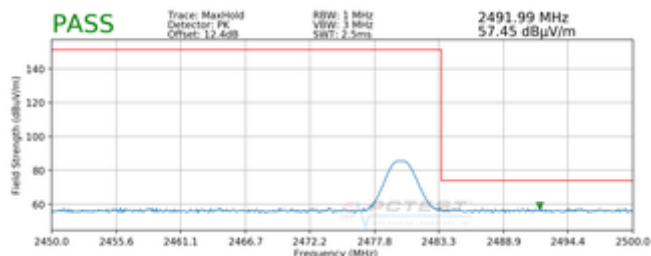
Plot 7-21. Radiated Restricted Upper Band Edge Measurement (Peak - Closed)
