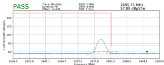
Plot 7-19. Radiated Restricted Upper Band Edge Measurement (Peak - Open)
