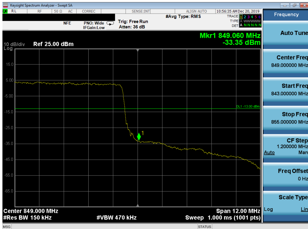
Plot 7-128. Upper Band Edge Plot (Band 26 - 15.0MHz QPSK - Full RB Configuration)
