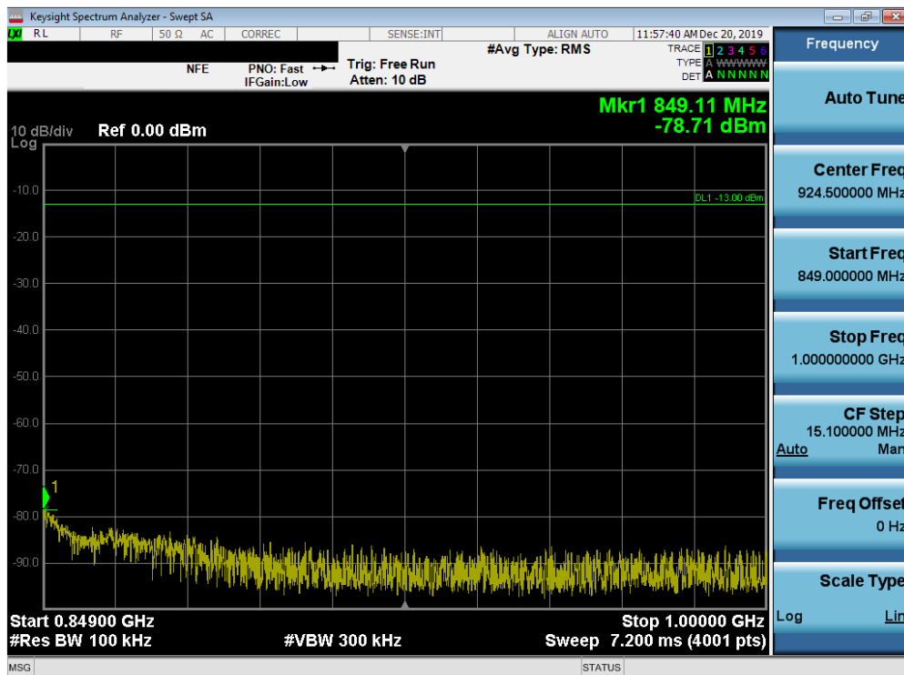
Plot 7-12. Conducted Spurious Plot (LTE Band 26 - 5MHz QPSK - RB Size 1, RB Offset 0 - Low Channel)
