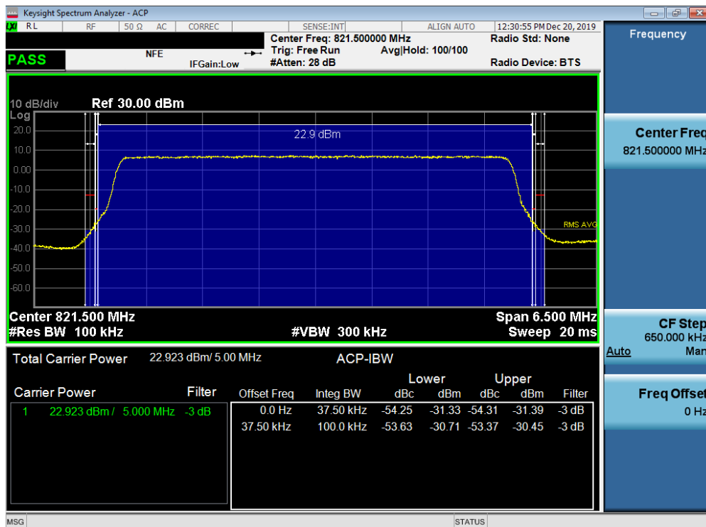
Plot 7-22. Channel Edge Plot (LTE Band 26 - 5MHz QPSK - High Channel)
