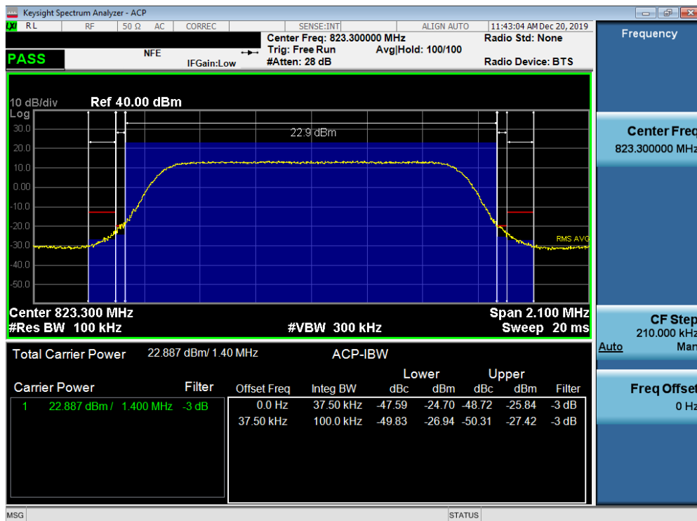
Plot 7-18. Channel Edge Plot (LTE Band 26 - 1.4MHz QPSK - High Channel)
