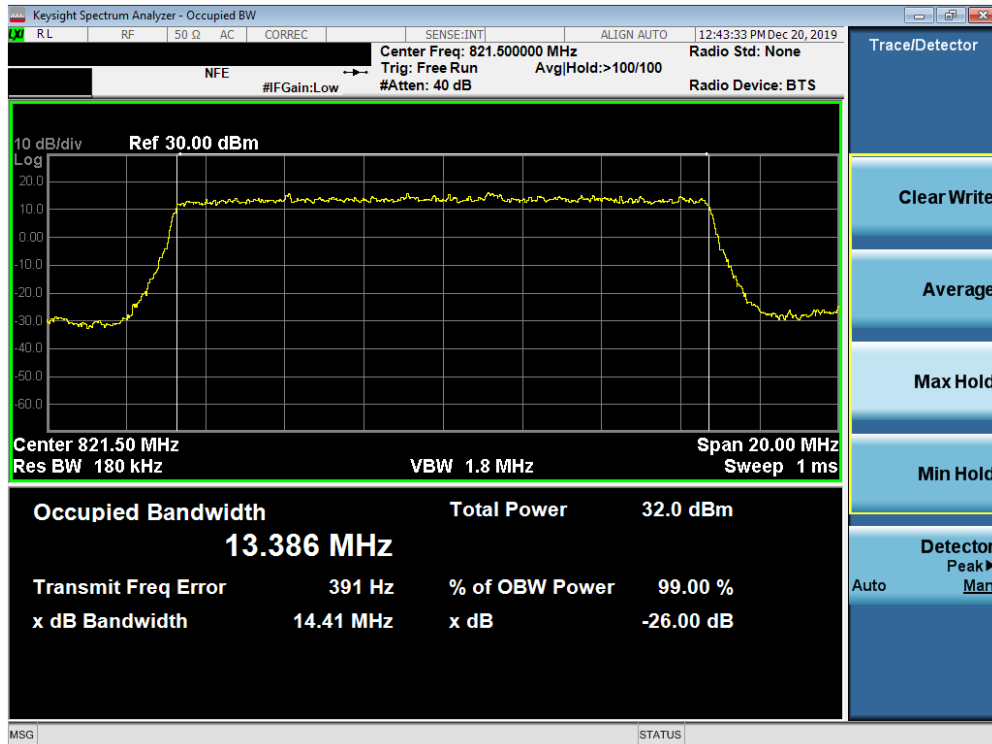
Plot 7-9. Occupied Bandwidth Plot (LTE Band 26 - 15MHz QPSK - Full RB Configuration)
