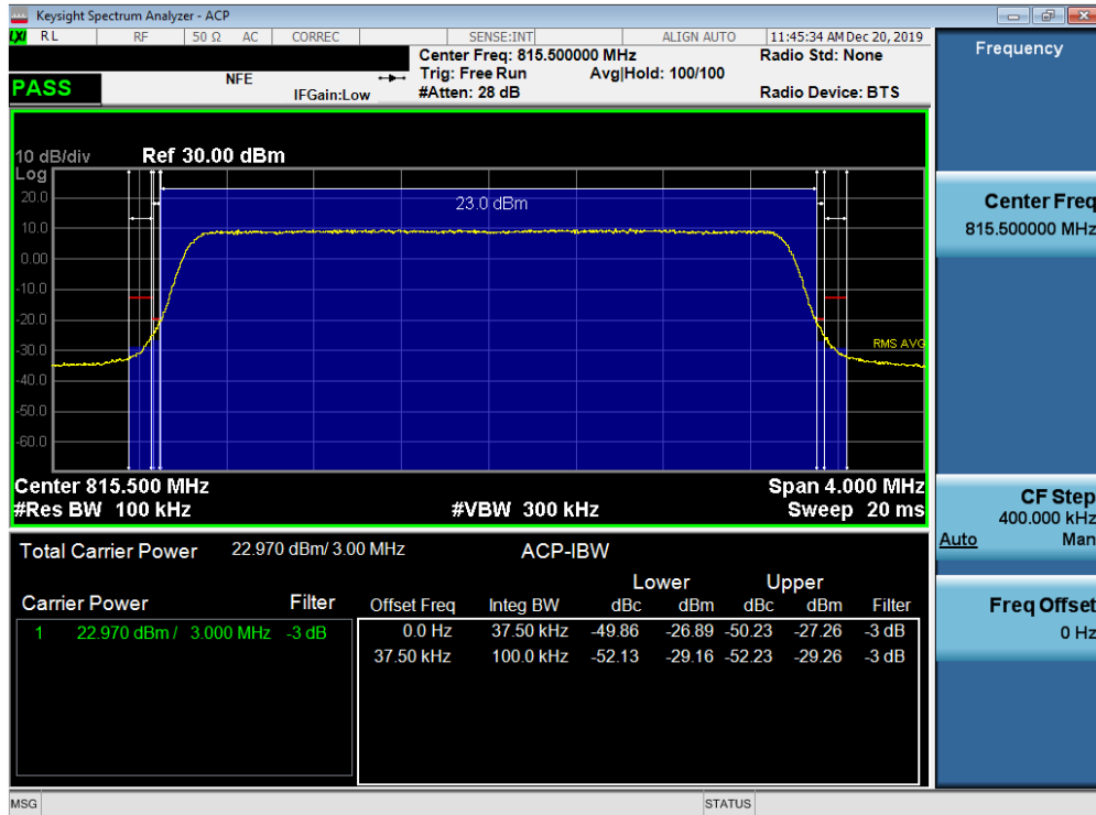
Plot 7-19. Channel Edge Plot (LTE Band 26 - 3MHz QPSK - Low Channel)
