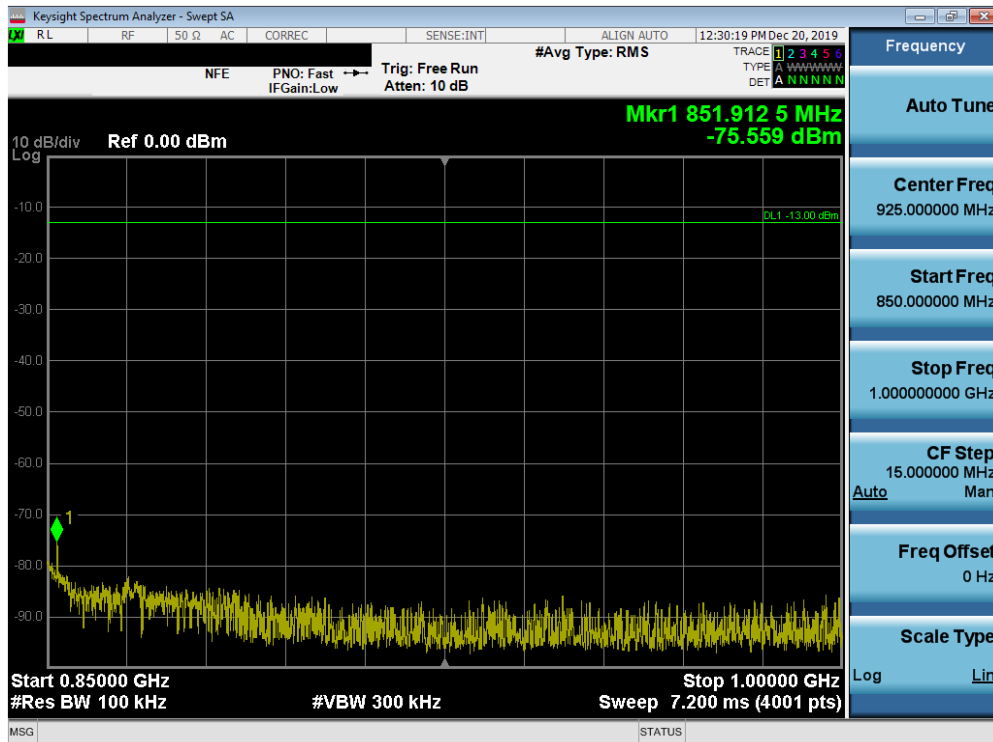
Plot 7-15. Conducted Spurious Plot (LTE Band 26 - 5MHz QPSK - RB Size 1, RB Offset 0 - High Channel)
