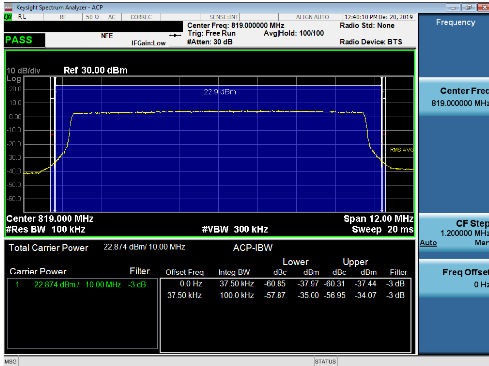
Plot 7-23. Channel Edge Plot (LTE Band 26 - 10MHz QPSK - Low Channel)
