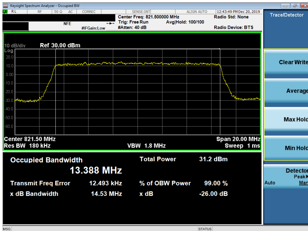
Plot 7-10. Occupied Bandwidth Plot (LTE Band 26 - 15MHz 16-QAM - Full RB Configuration)
