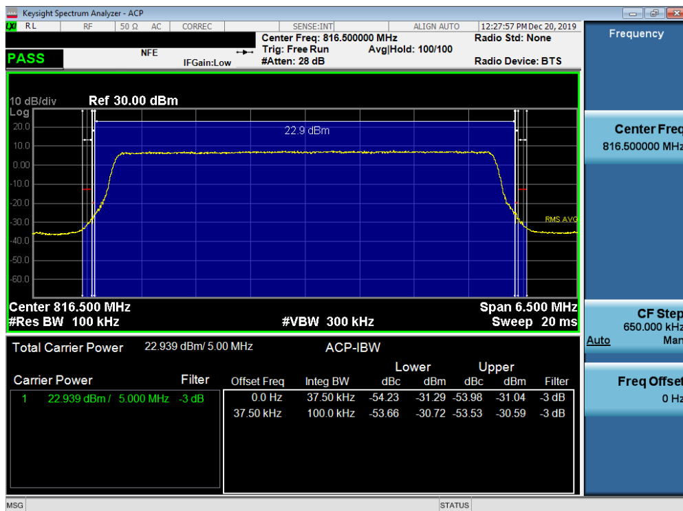
Plot 7-21. Channel Edge Plot (LTE Band 26 - 5MHz QPSK - Low Channel)
