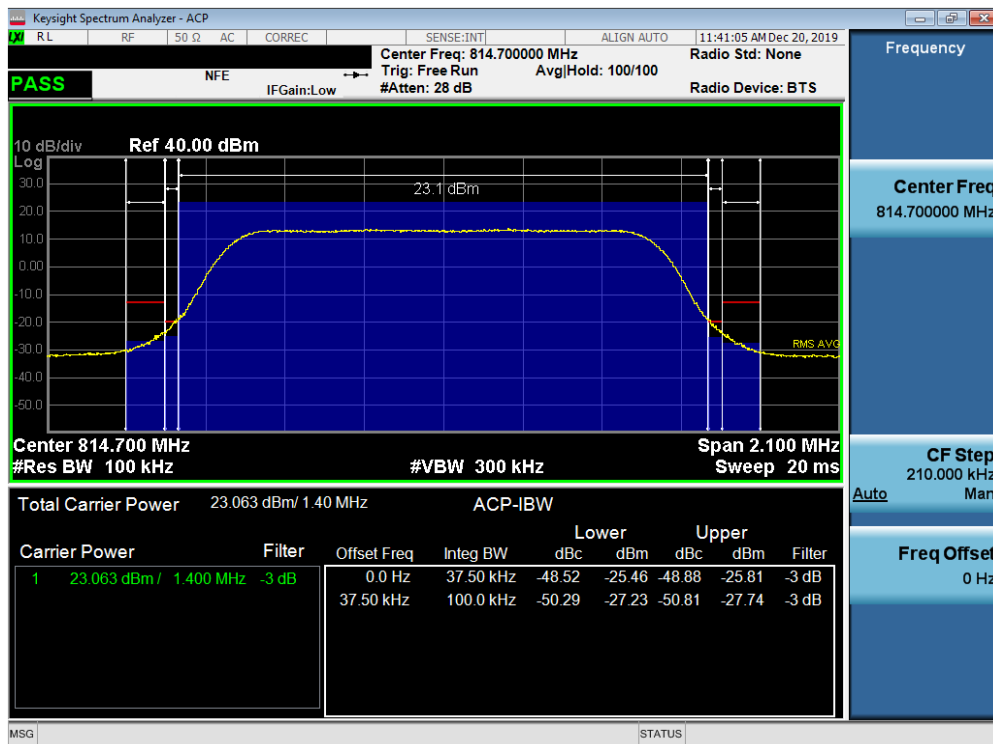
Plot 7-17. Channel Edge Plot (LTE Band 26 - 1.4MHz QPSK - Low Channel)
