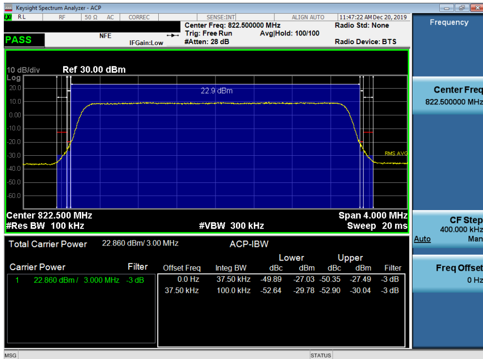
Plot 7-20. Channel Edge Plot (LTE Band 26 - 3MHz QPSK - High Channel)
