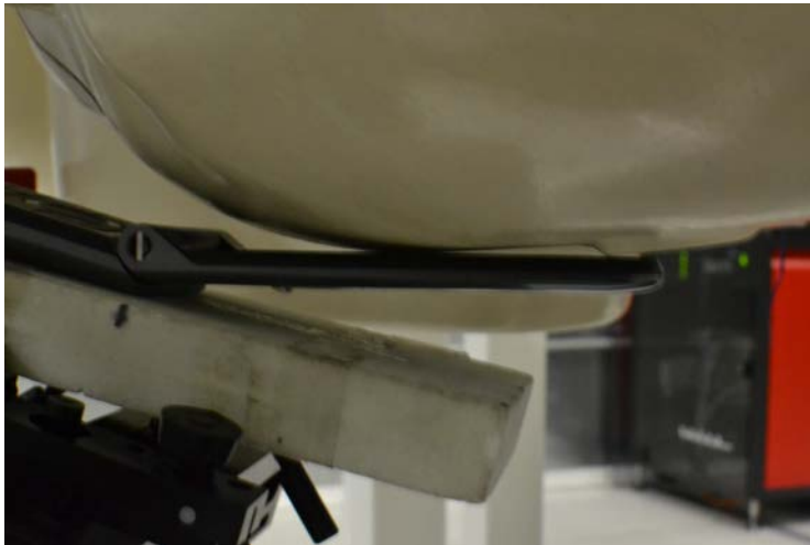
SAR Test Setup Photo 4 – Left Cheek
