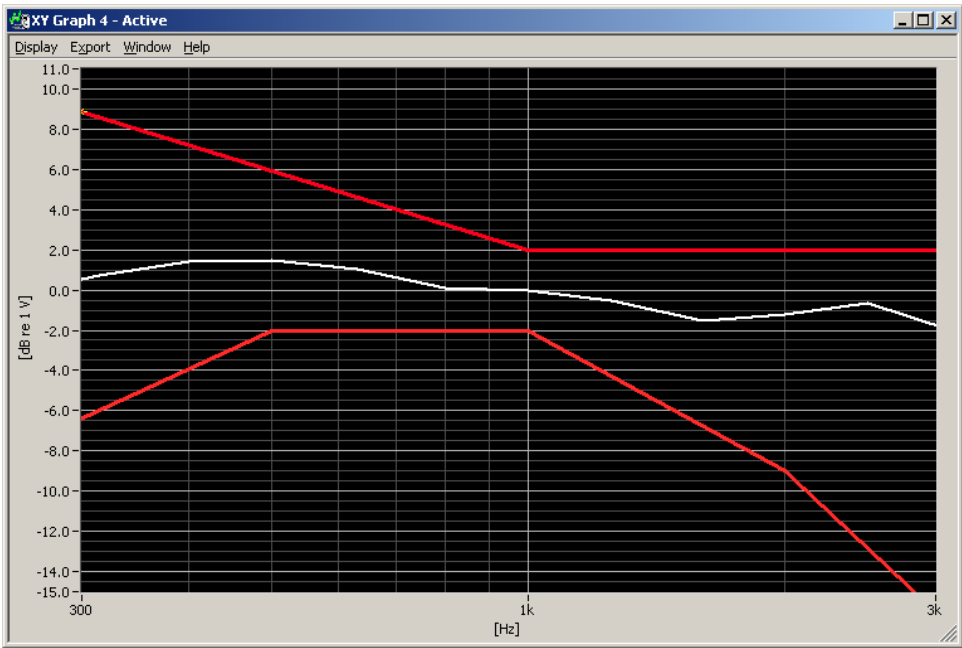
Figure 6-1 Axial Frequency Response
