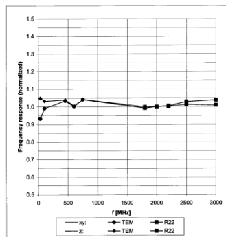
Figure 5-2 E-Field Probe Frequency Response
