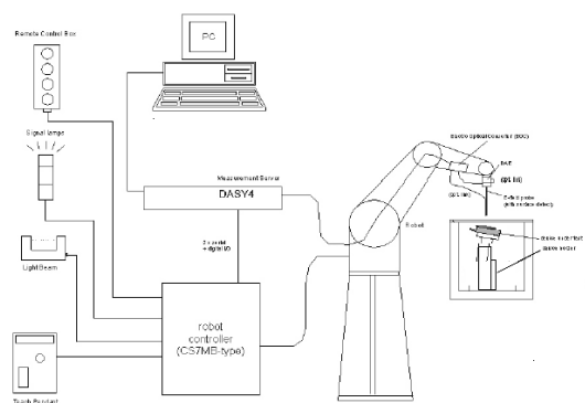
Figure 5-4 SPEAG Robotic System Diagram
