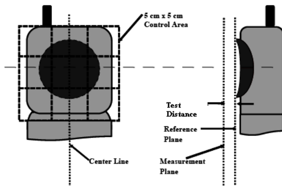
Figure 6-2 E-Field Emissions Test Setup Diagram (See Test Photographs for actual WD scan grid overlay)
