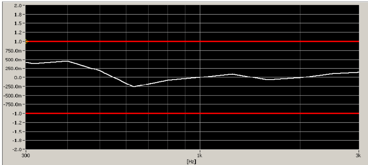
Figure 7-3 Helmholtz Coil Validation for Frequency Response
