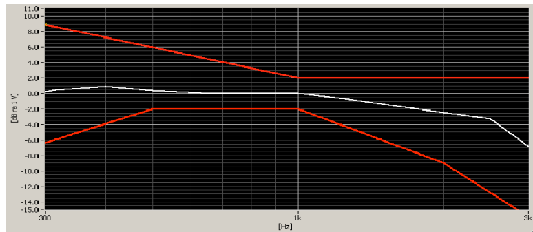
Figure 7-1 Axial Frequency Response
