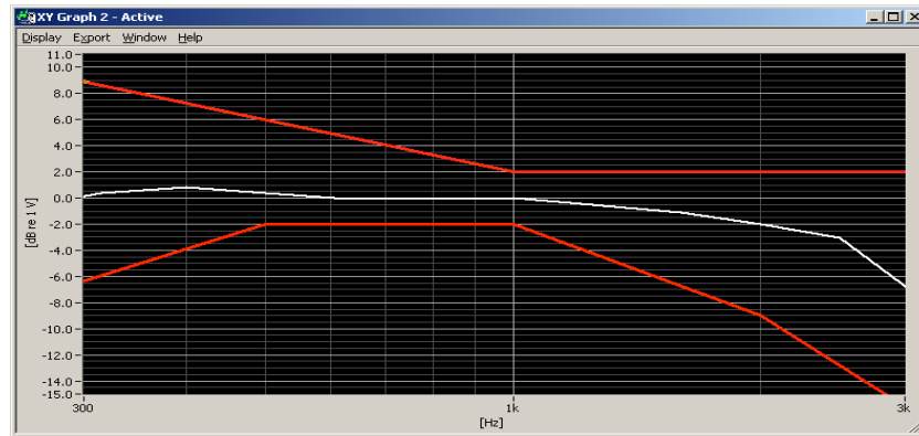
Figure 6-1 Axial Frequency Response
