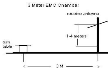
Figure 6-6. Test Instrument & Measurement Setup
