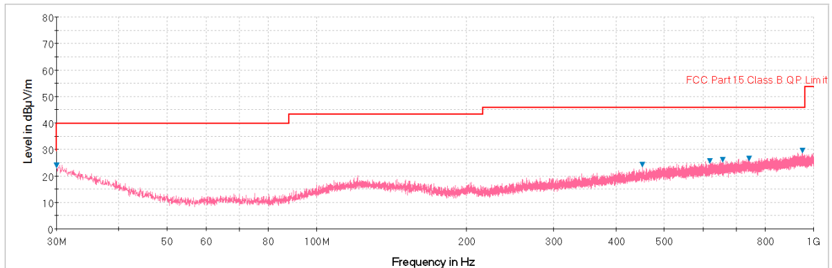
Plot 7-50. Radiated Spurious Plot below 1GHz (Pol. H)
