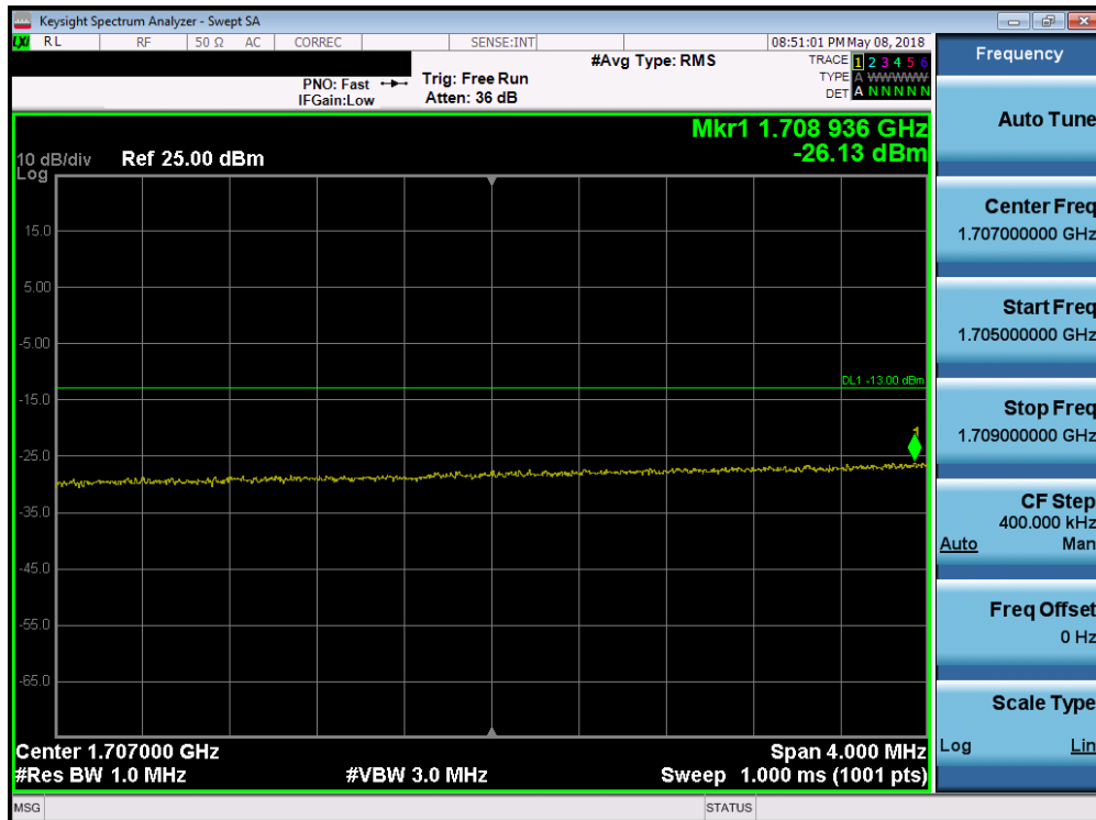
Plot 7-149. Lower Extended Band Edge Plot (Band 66/4 - 20.0MHz QPSK - Full RB Configuration)
