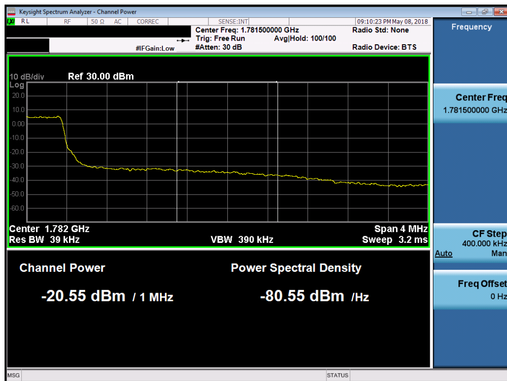
Plot 7-129. Upper Extended Band Edge Plot (Band 66 - 3.0MHz QPSK - Full RB Configuration)
