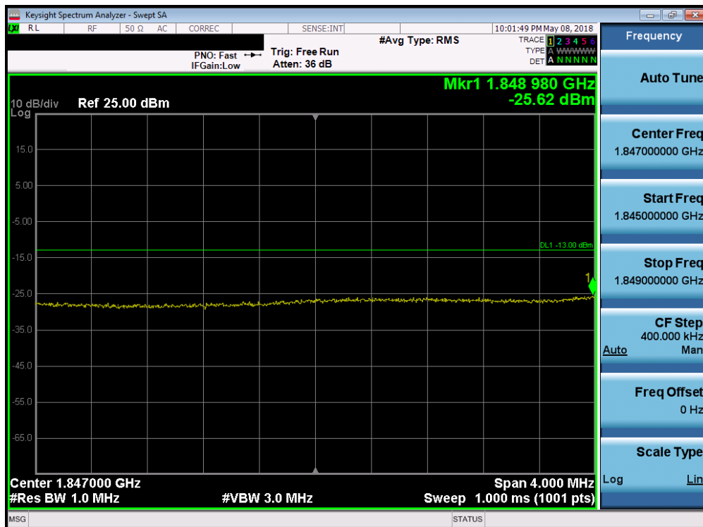
Plot 7-171. Lower Extended Band Edge Plot (Band 2 - 15.0MHz QPSK - Full RB Configuration)
