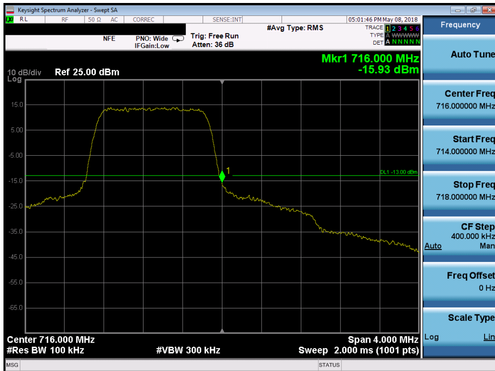
Plot 7-103. Upper Band Edge Plot (Band 12 - 1.4MHz QPSK - Full RB Configuration)
