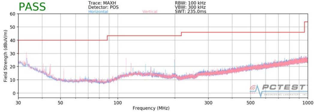
Plot 7-48. Radiated Spurious Plot below 1GHz GFSK
