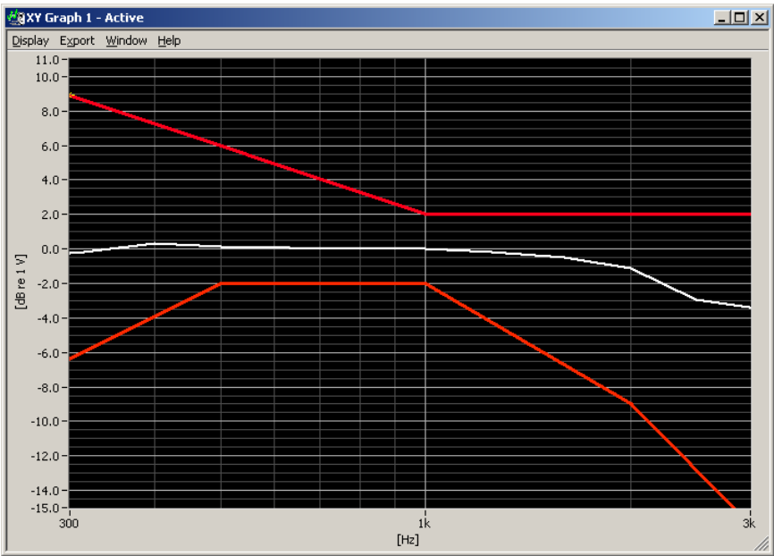
Figure 6-1 Axial Frequency Response
