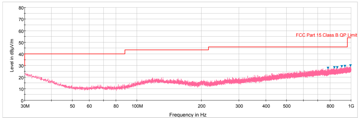
Plot 6-51. Radiated Spurious Plot below 1GHz (Pol. V)
