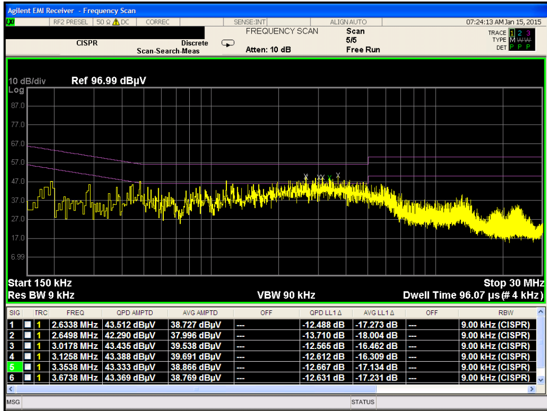
Plot 6-54. Line-Conducted Test Plot (L1)
