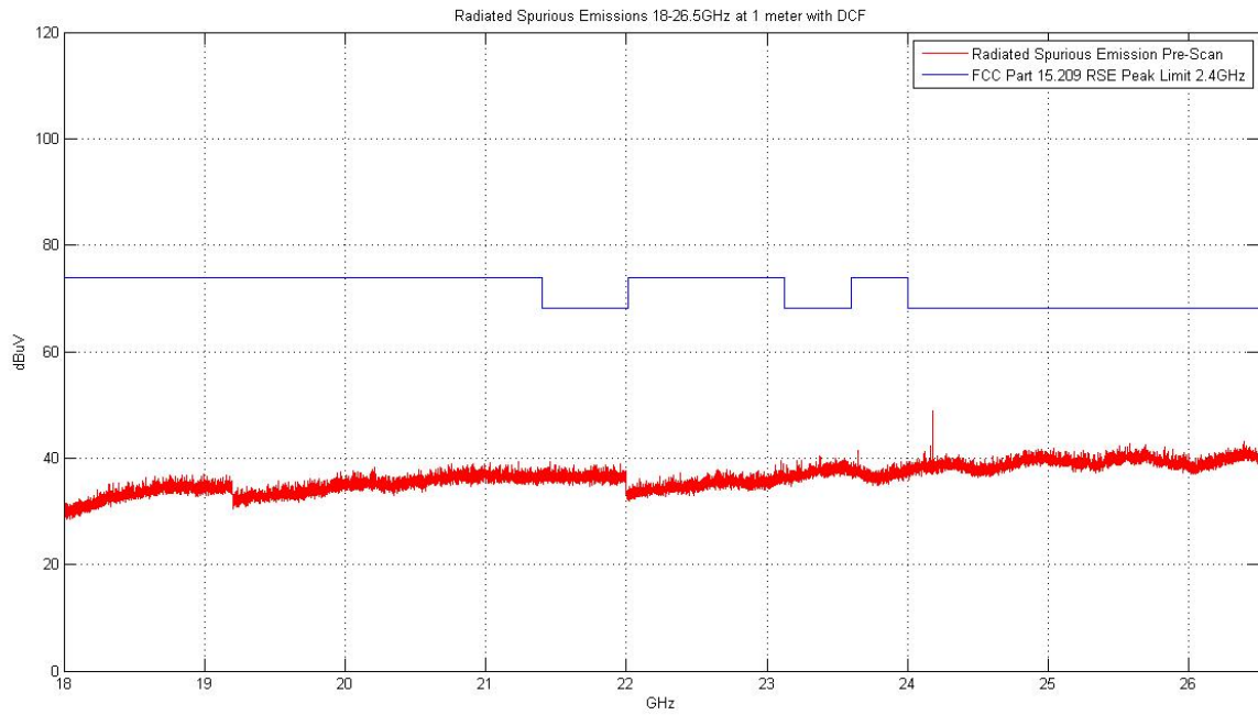
Plot 6-52. Radiated Spurious Plot above 18GHz (Pol. H)
