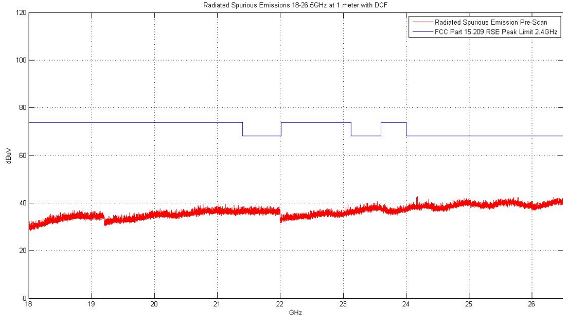
Plot 6-53. Radiated Spurious Plot above 18GHz (Pol. V)
