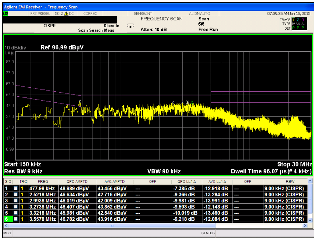
Plot 6-55. Line-Conducted Test Plot (N)
