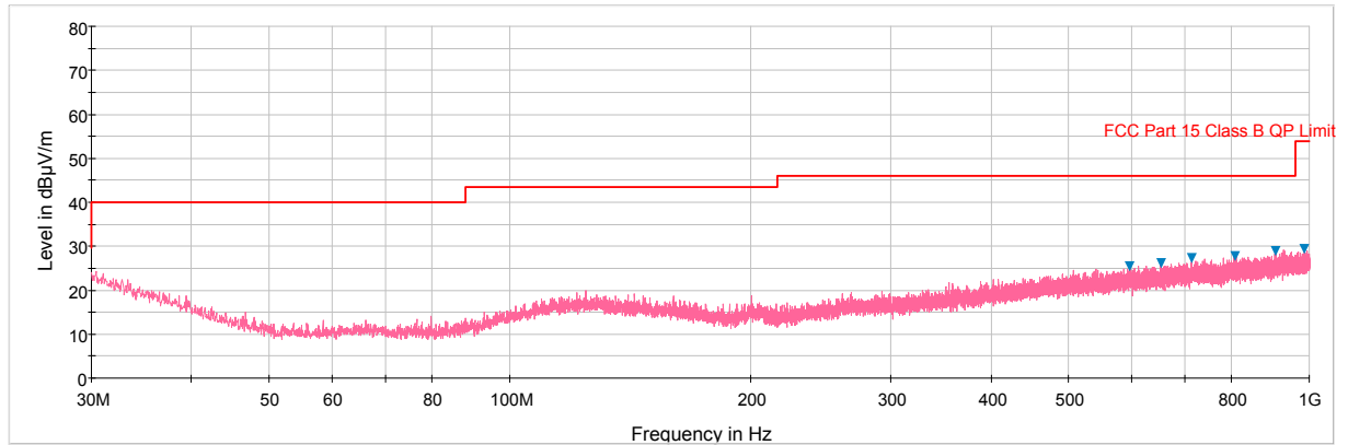
Plot 6-50. Radiated Spurious Plot below 1GHz (Pol. H)
