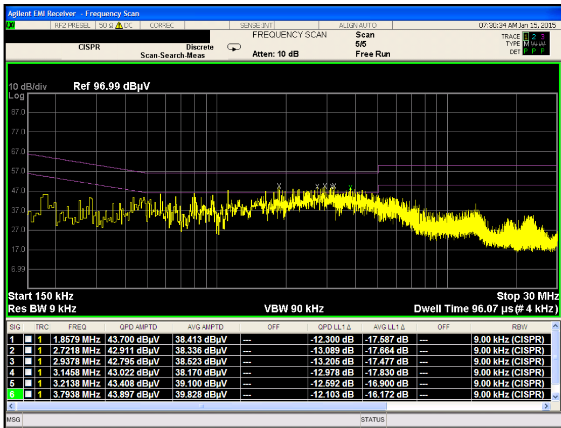
Plot 6-35. Line Conducted Plot with 802.11b (L1)
