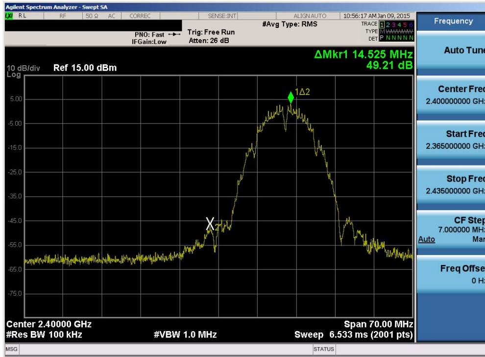
Plot 6-19. Band Edge Plot (802.11b – Ch. 1)
