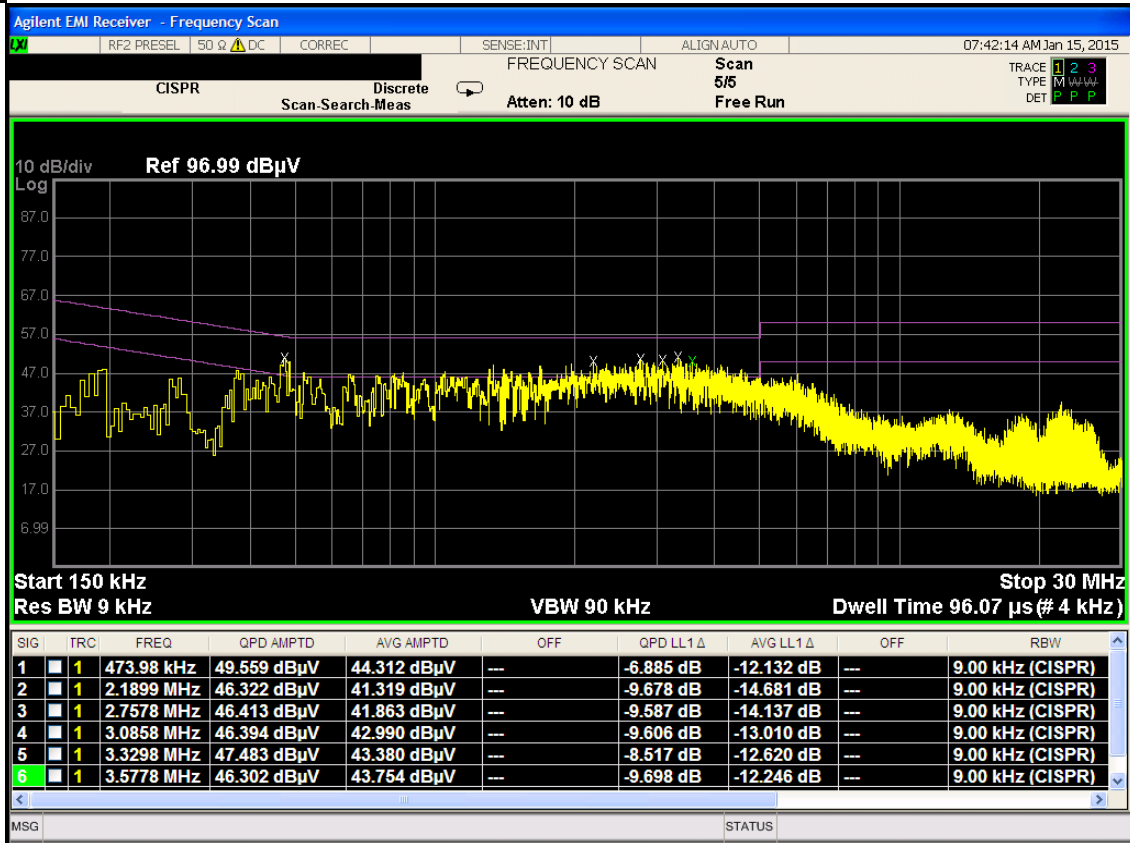
Plot 6-36. Line Conducted Plot with 802.11b (N)
