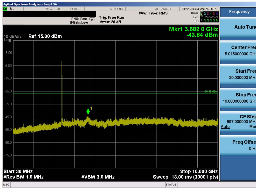
Plot 6-25. Conducted Spurious Plot (802.11b – Ch. 1)
