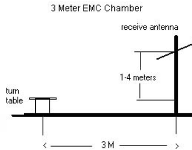
Figure 6-1. Test Instrument & Measurement Setup
