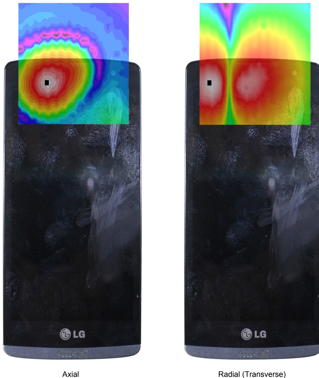
Figure 13-3 T-Coil Scan Overlay Magnetic Field Distributions
