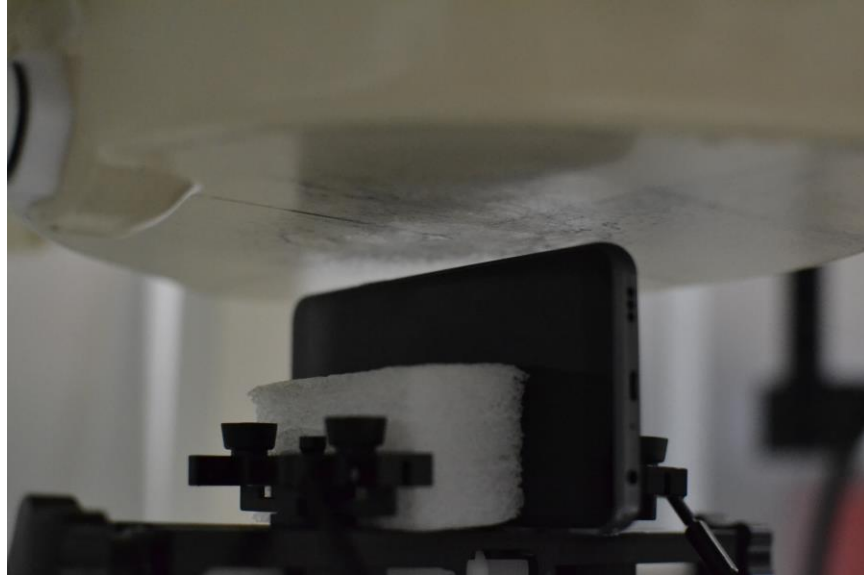
SAR Test Setup Photo 6 – Right Edge at 10mm
