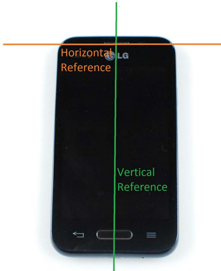
SAR Test Setup Photo 11 - Vertical and Horizontal Reference Lines
