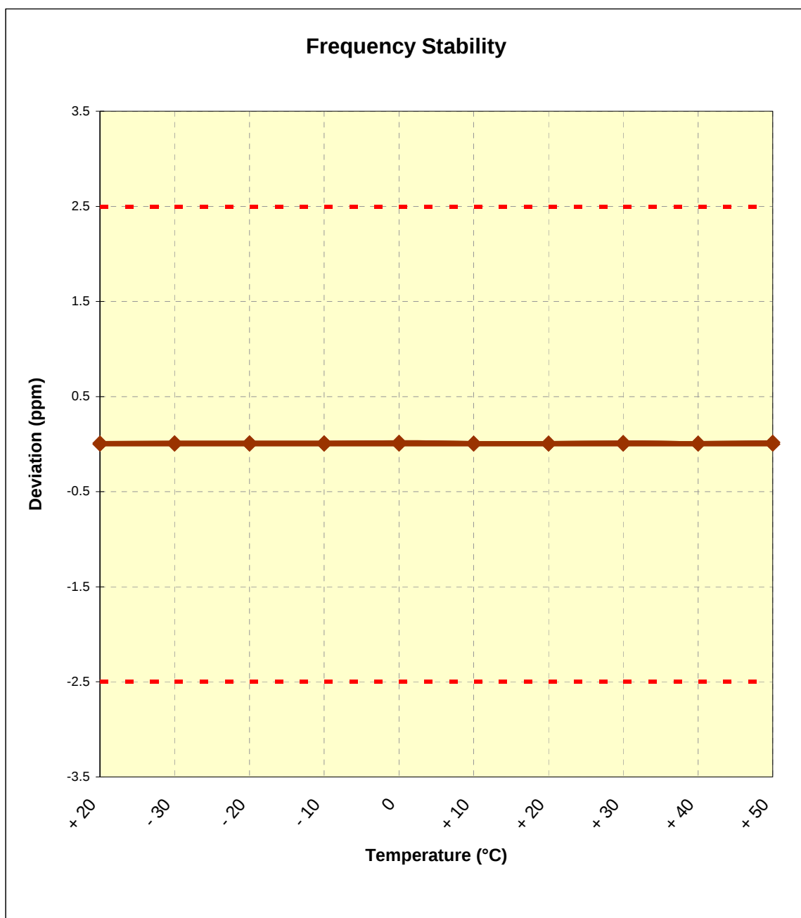
Figure 6-1. Frequency Stability Graph (Cellular CDMA Mode – Ch. 384)
