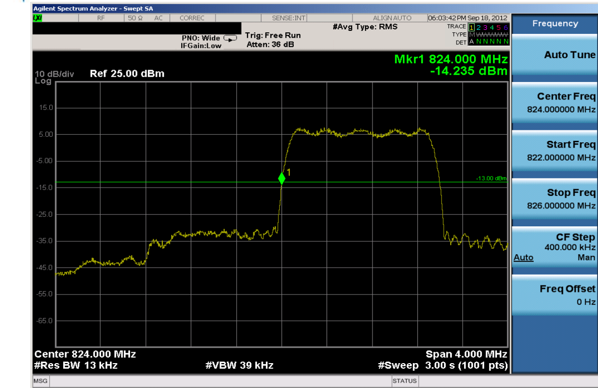
Plot 7-3. Band Edge Plot (Cellular CDMA Mode – Ch. 1013)
