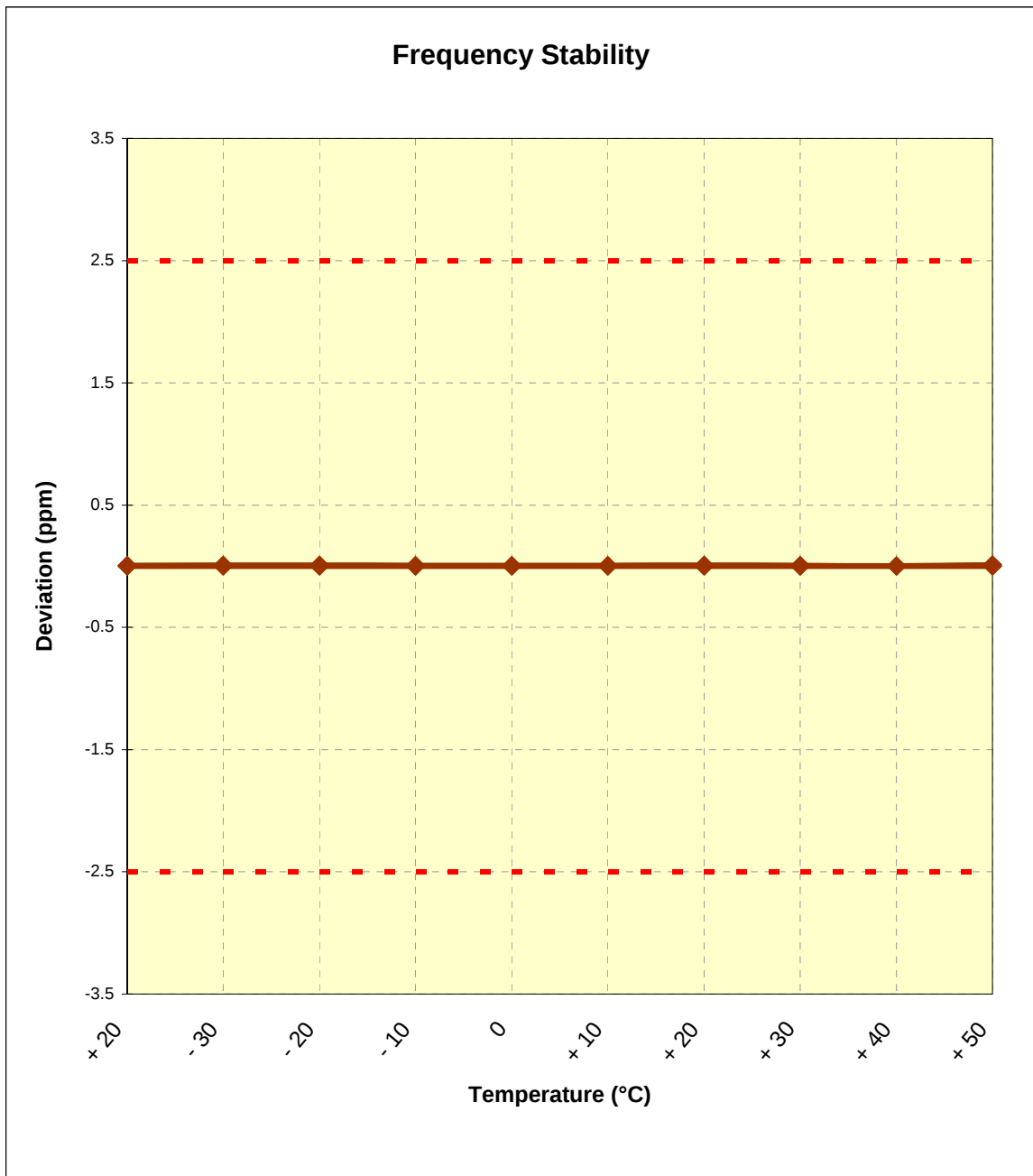
Figure 6-2. Frequency Stability Graph (PCS CDMA Mode – Ch. 600)
