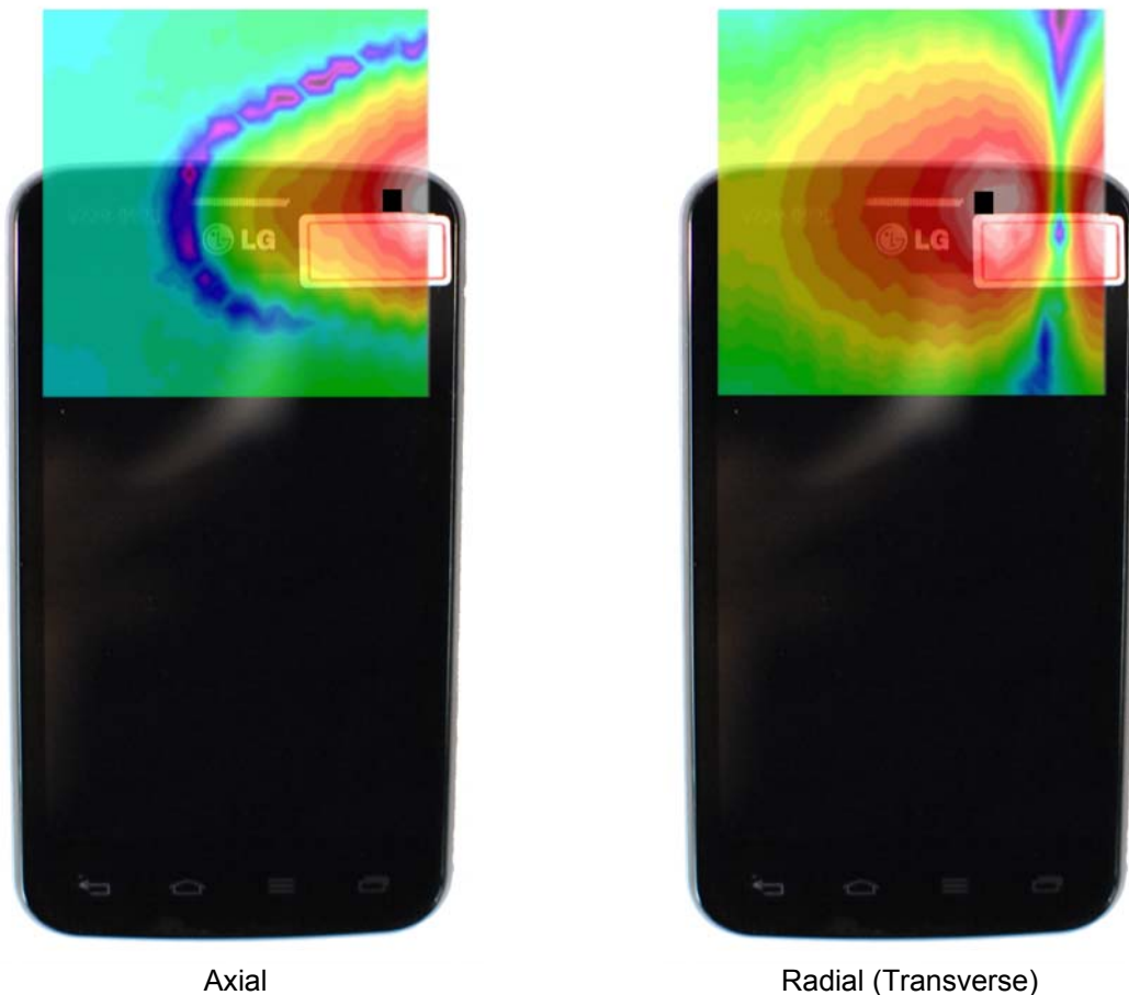
Axial Radial (Transverse) Figure 13-3 T-Coil Scan Overlay Magnetic Field Distributions
