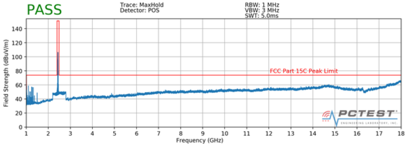
Plot 7-34. Radiated Spurious Plot above 1GHz (802.11b – Ch. 6, Ant. Pol. V)
