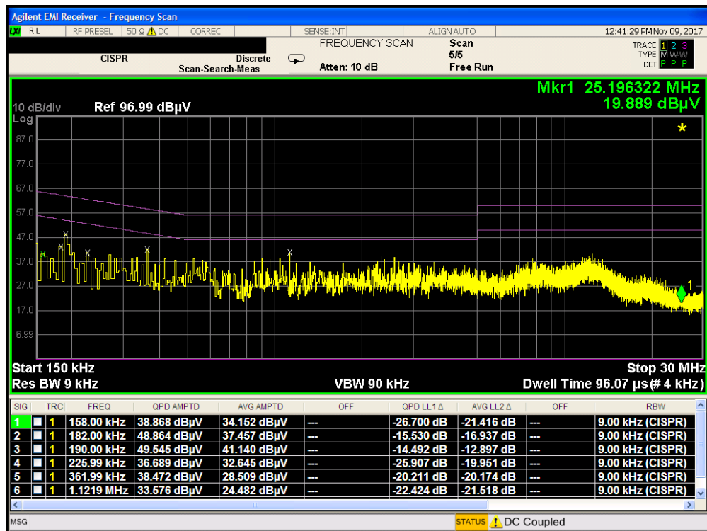
Plot 7-49. Line Conducted Plot with 802.11b (L1)
