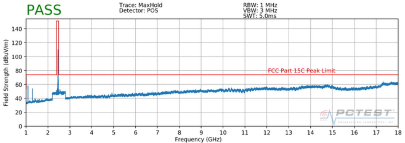
Plot 7-36. Radiated Spurious Plot above 1GHz (802.11b – Ch. 11, Ant. Pol. V)
