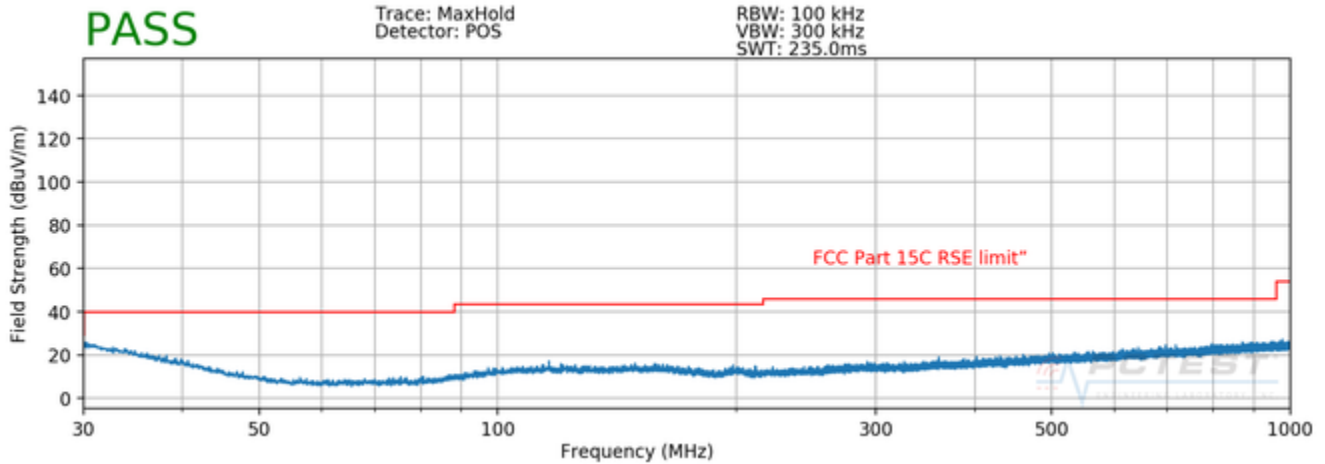
Plot 7-48. Radiated Spurious Plot below 1GHz (Pol. V)
