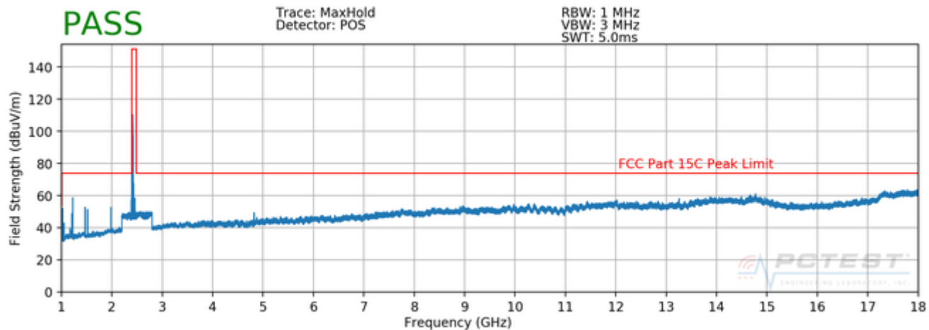
Plot 7-32. Radiated Spurious Plot above 1GHz (802.11b – Ch. 1, Ant. Pol. V)
