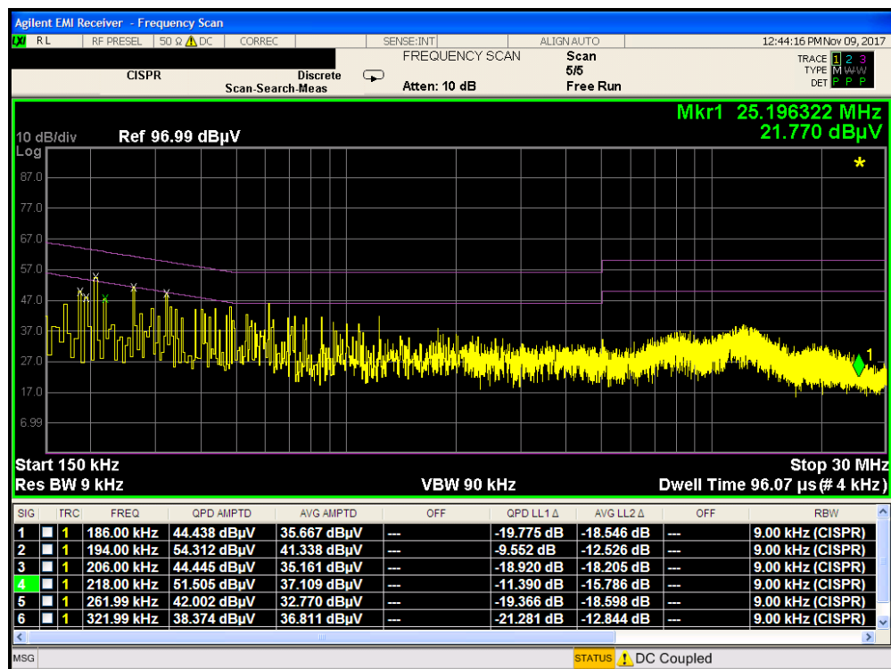
Plot 7-50. Line Conducted Plot with 802.11b (N)
