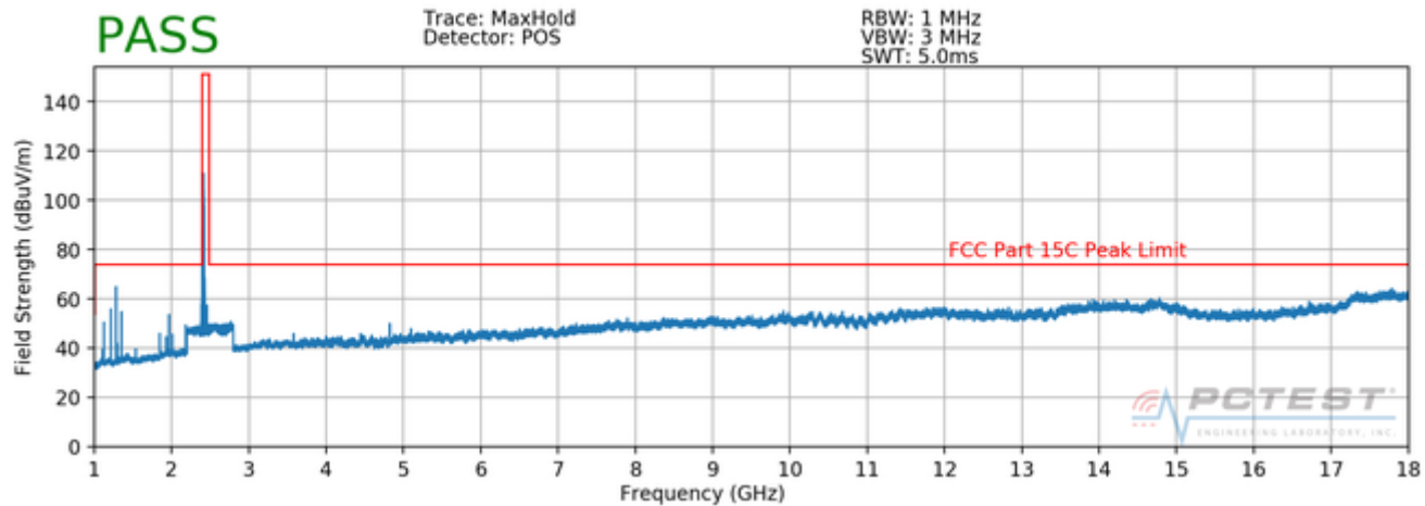
Plot 7-31. Radiated Spurious Plot above 1GHz (802.11b – Ch. 1, Ant. Pol. H)
