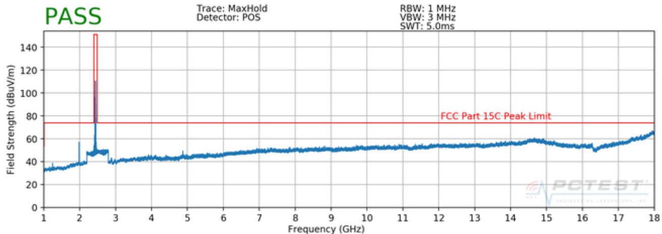
Plot 7-33. Radiated Spurious Plot above 1GHz (802.11b – Ch. 6, Ant. Pol. H)
