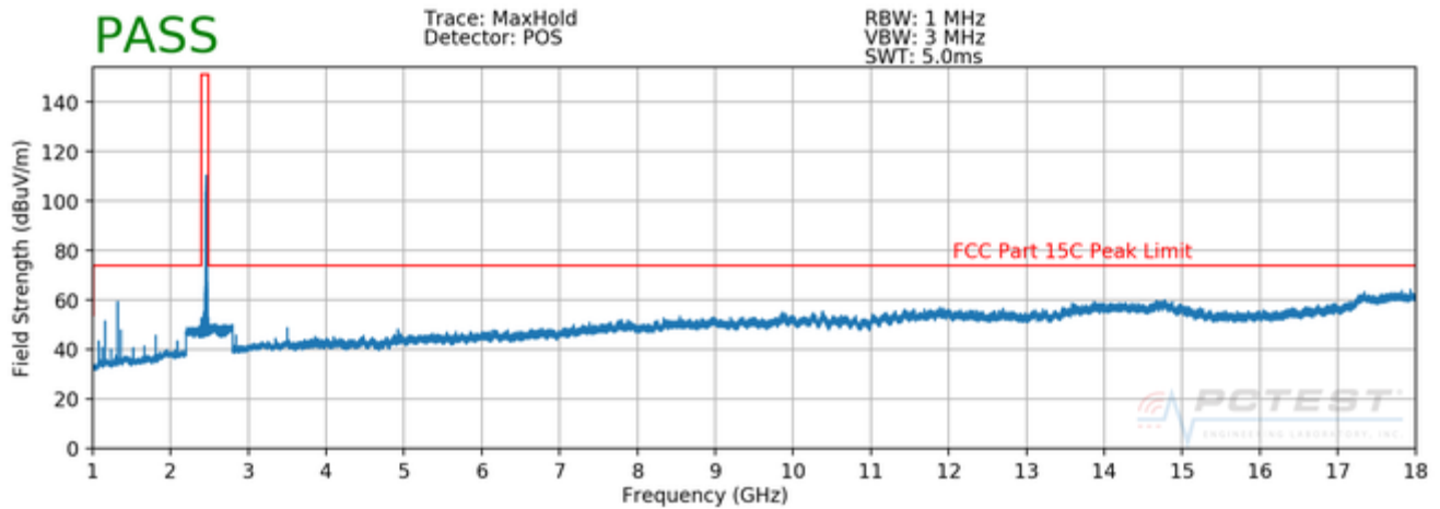
Plot 7-35. Radiated Spurious Plot above 1GHz (802.11b – Ch. 11, Ant. Pol. H)
