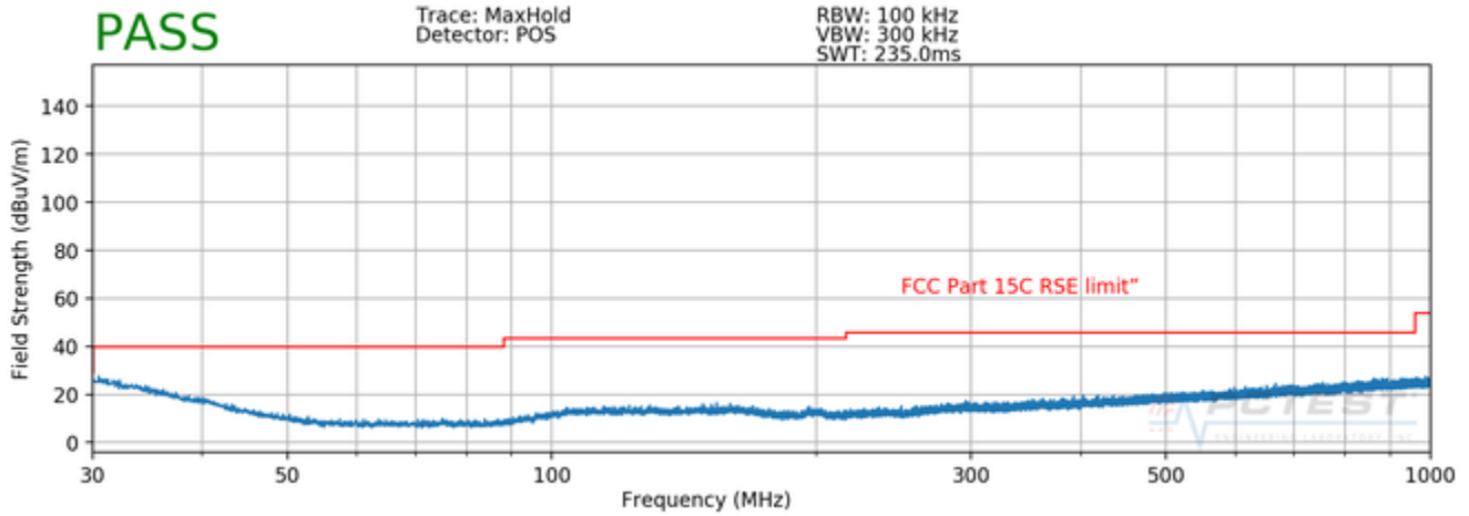
Plot 7-47. Radiated Spurious Plot below 1GHz (Pol. H)
