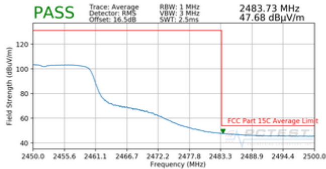
Plot 7-13. Radiated Restricted Upper Band Edge Measurement (Average)
