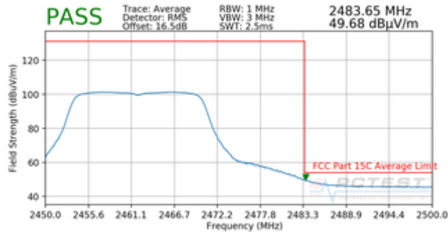
Plot 7-15. Radiated Restricted Upper Band Edge Measurement (Average)
