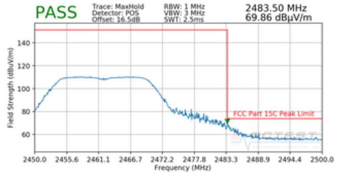
Plot 7-16. Radiated Restricted Upper Band Edge Measurement (Peak)
