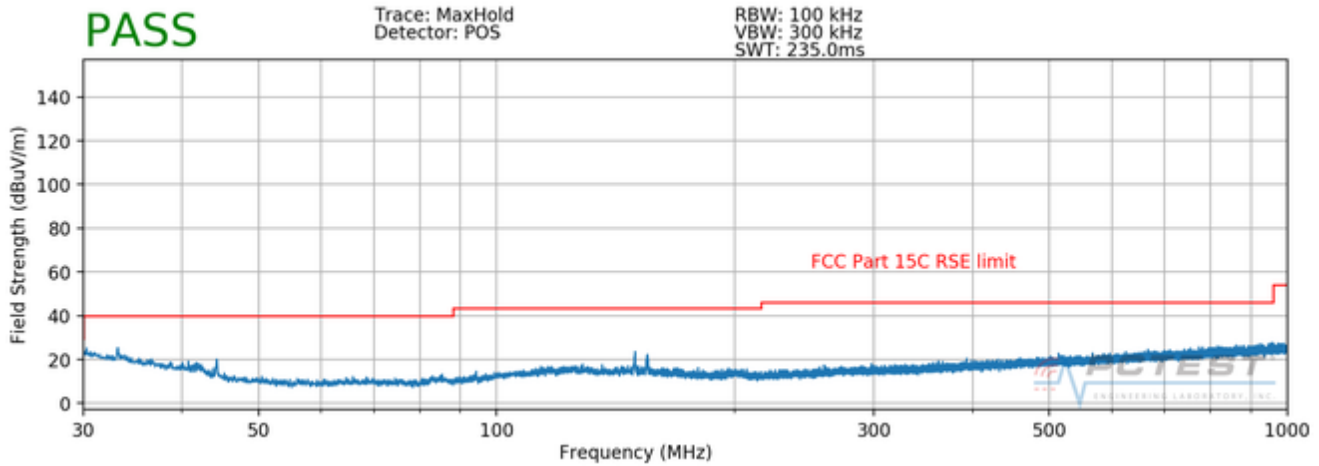
Plot 7-18. Radiated Spurious Plot below 1GHz (Pol. V)
