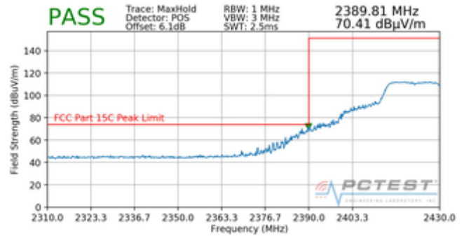
Plot 7-12. Radiated Restricted Lower Band Edge Measurement (Peak)
