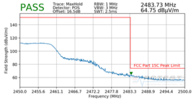
Plot 7-14. Radiated Restricted Upper Band Edge Measurement (Peak)
