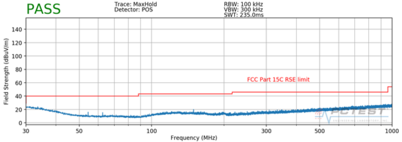
Plot 7-17. Radiated Spurious Plot below 1GHz (Pol. H)
