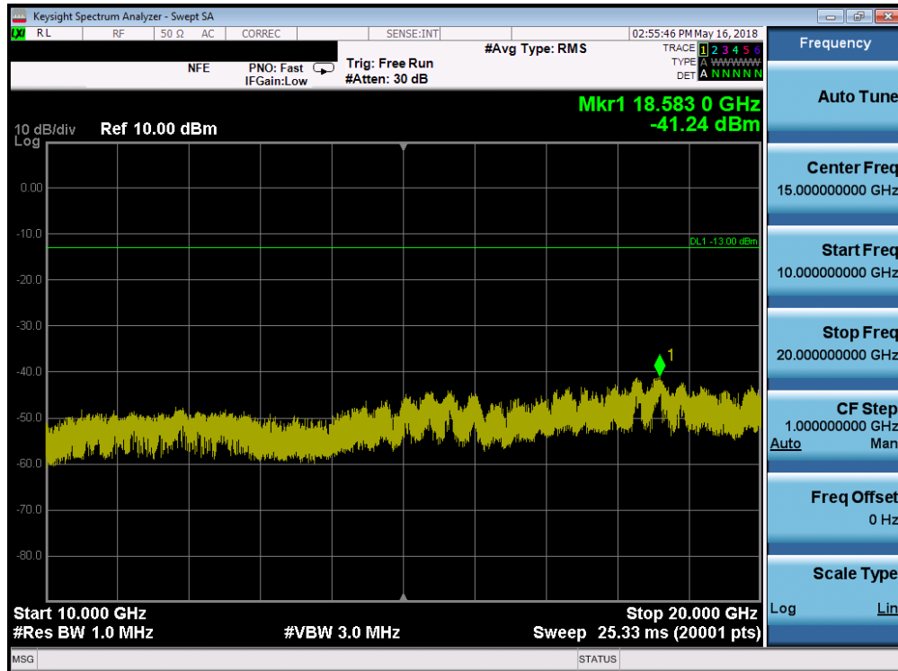
Plot 7-106. Conducted Spurious Plot (Band 2 - 20.0MHz QPSK - RB Size 1, RB Offset 0 - High Channel)
