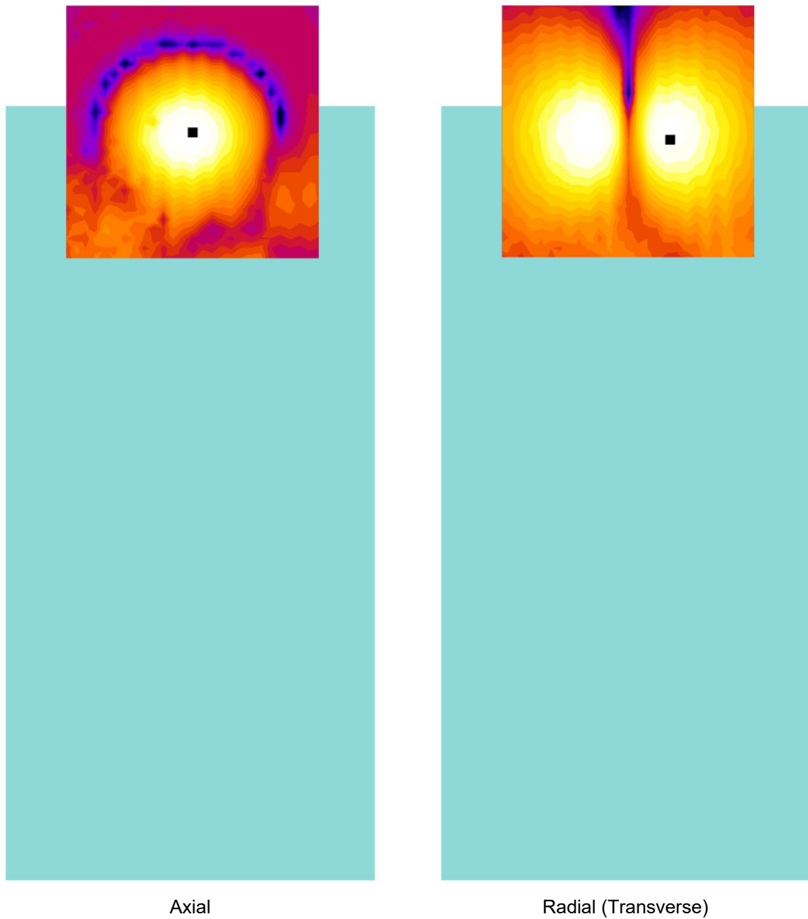
Figure 9-2 T-Coil Scan Overlay Magnetic Field Distributions (OTT VoIP Testing)
