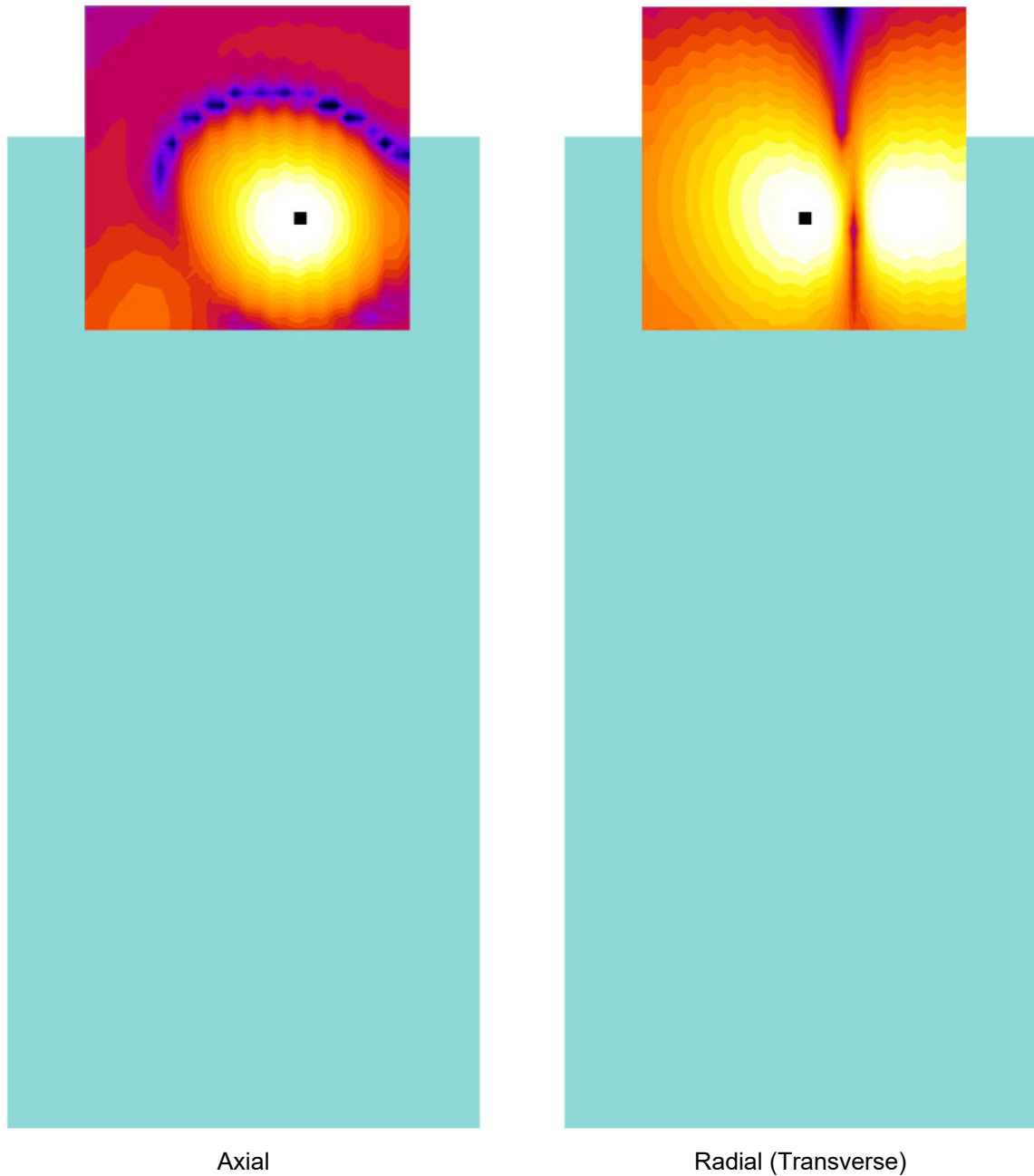
Figure 9-1 T-Coil Scan Overlay Magnetic Field Distributions (CMRS Testing)
