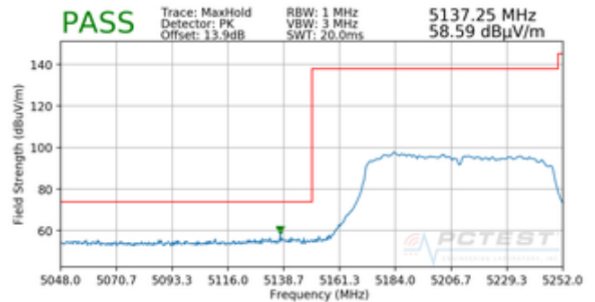
Plot 7-100. Radiated Lower Band Edge Plot (Peak – UNII Band 1)
