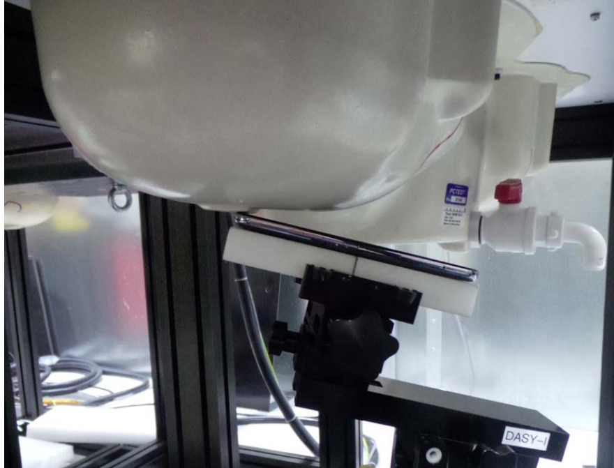
SAR Test Setup Photo 4: Right Tilt
