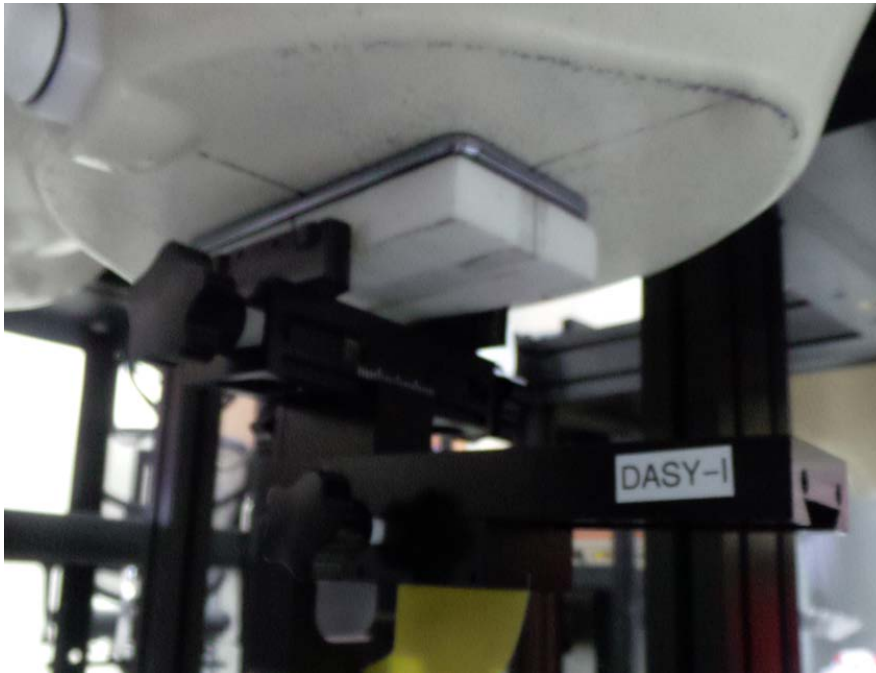
SAR Test Setup Photo 11: Front at 0.0 cm
