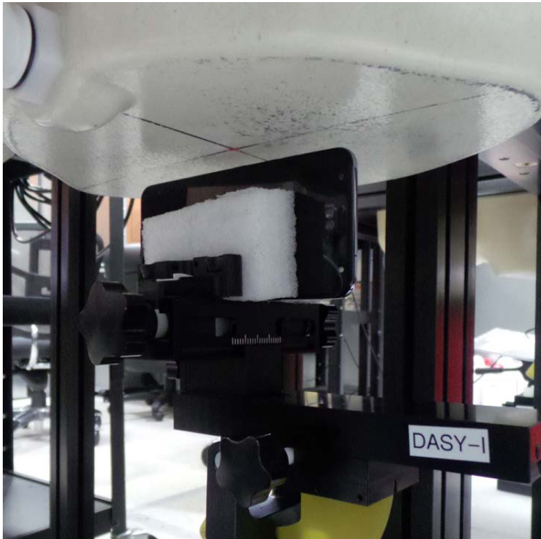
SAR Test Setup Photo 17: Left at 1.0 cm
