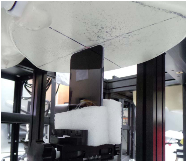
SAR Test Setup Photo 13: Bottom at 0.4 cm
