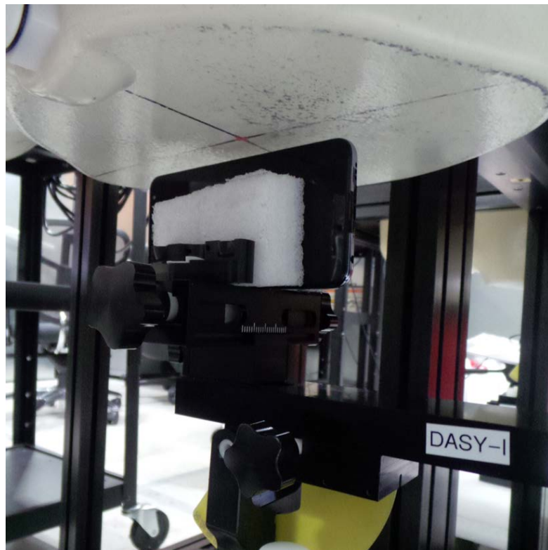
SAR Test Setup Photo 19: Right at 1.0 cm
