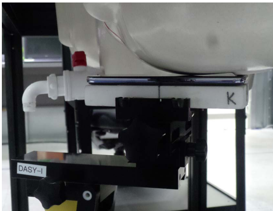
SAR Test Setup Photo 1: Left Cheek
