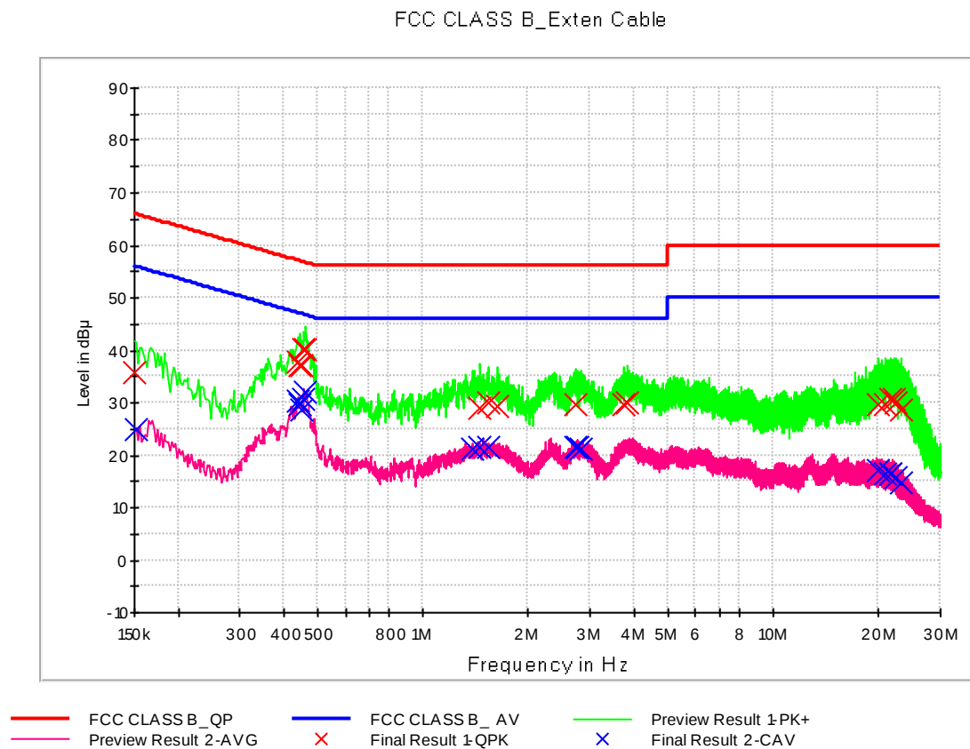
Figure 1: Conducted Emission (150 kHz to 30 MHz), Line (L1)
