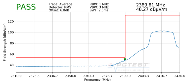
Plot 7-45. Radiated Restricted Lower Band Edge Measurement (Average)
