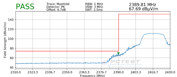
Plot 7-46. Radiated Restricted Lower Band Edge Measurement (Peak)
