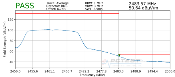
Plot 7-53. Radiated Restricted Upper Band Edge Measurement (Average)
