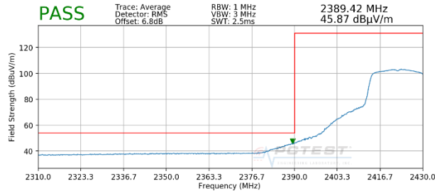
Plot 7-47. Radiated Restricted Lower Band Edge Measurement (Average)
