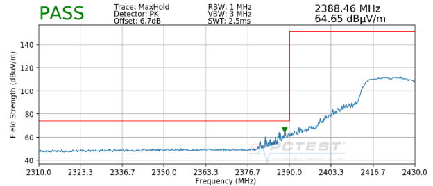
Plot 7-48. Radiated Restricted Lower Band Edge Measurement (Peak)
