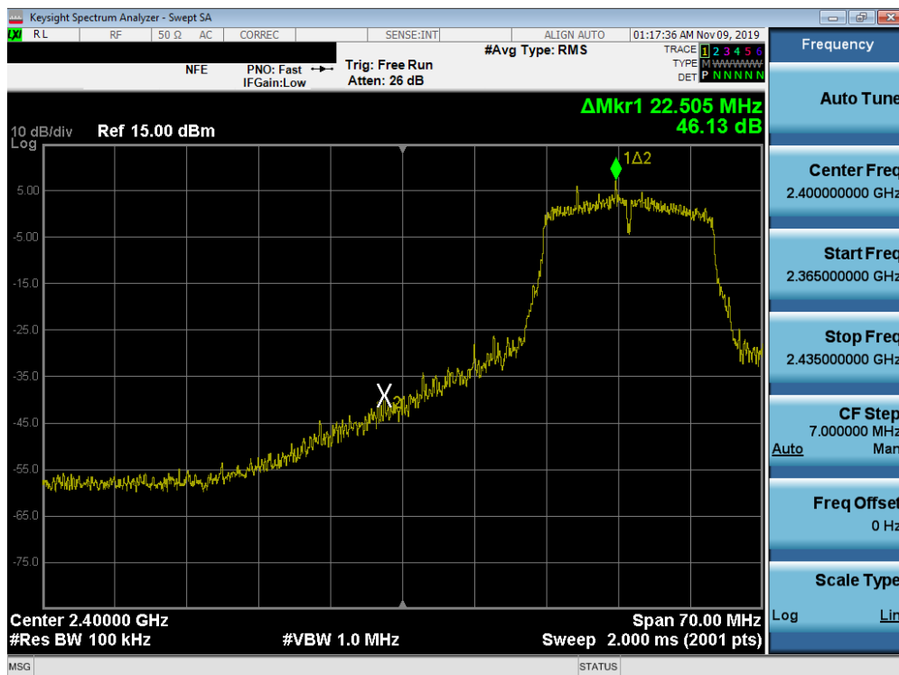
Plot 7-23. Band Edge Plot (802.11g– Ch. 3)
