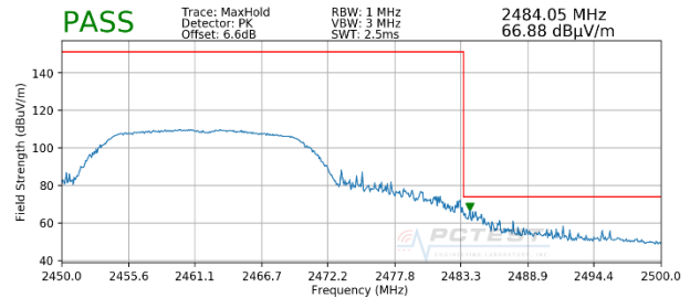
Plot 7-54. Radiated Restricted Upper Band Edge Measurement (Peak)
