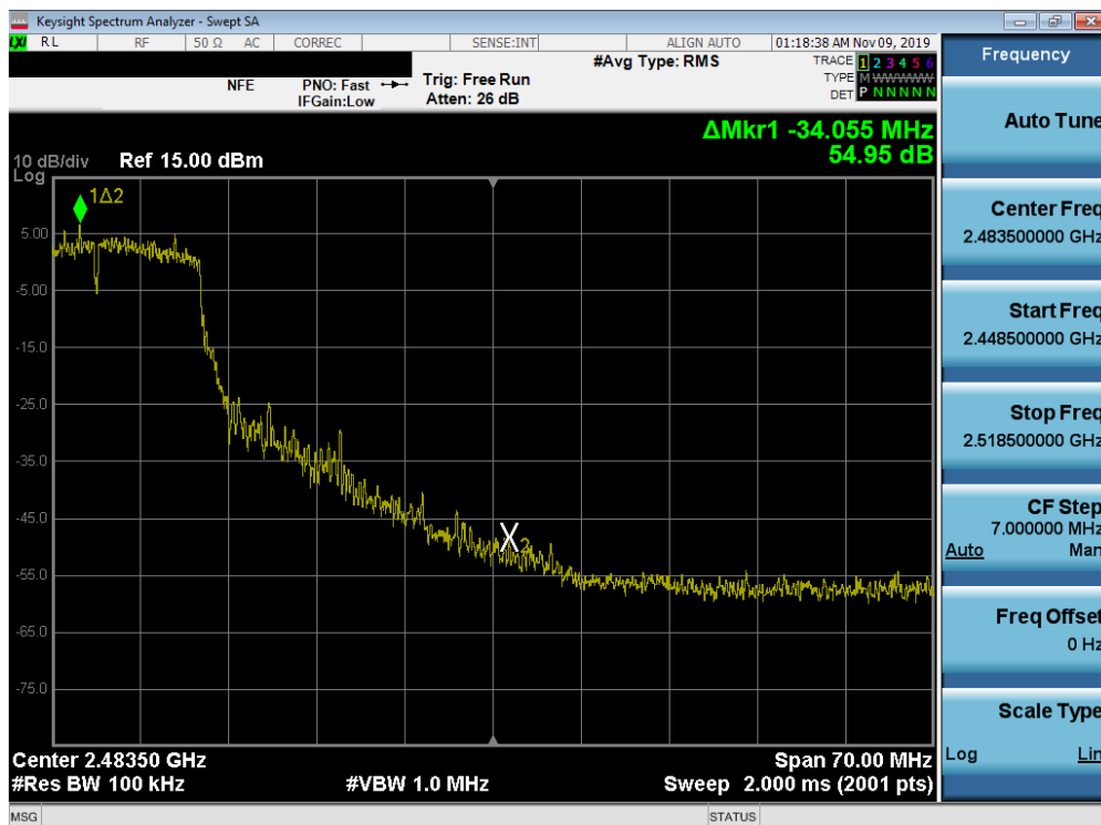
Plot 7-24. Band Edge Plot (802.11g – Ch. 9)
