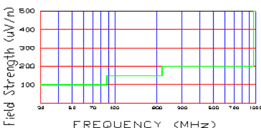
Figure 6-3. 3-Meter Limits
