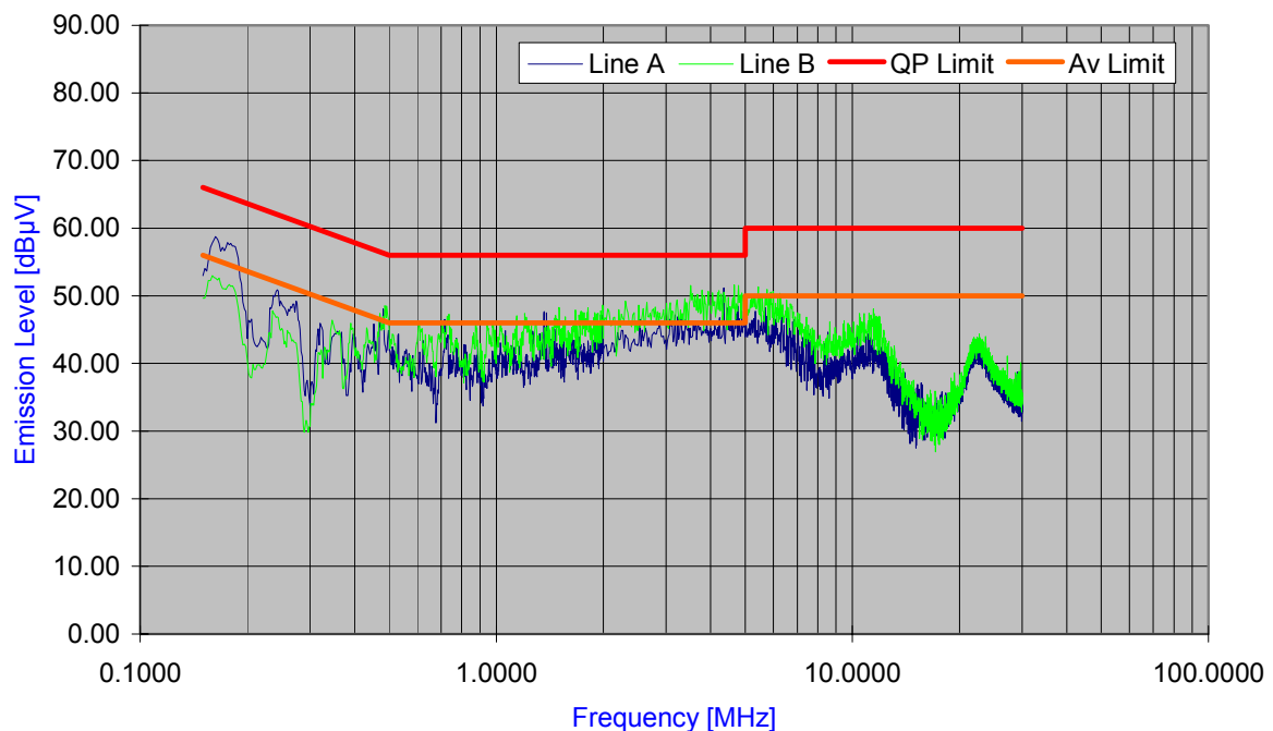
Plot 6-24. Line Conducted Plot with Bluetooth
