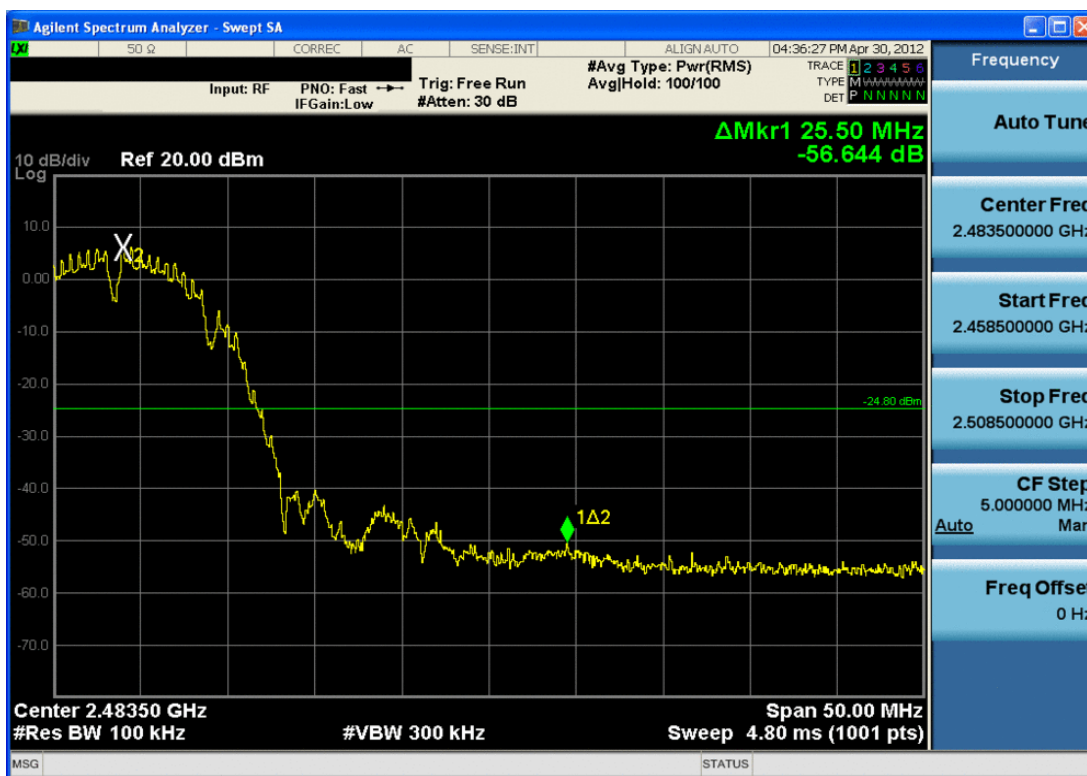
Plot 6-20. Band Edge Plot (802.11b – Ch. 11)
