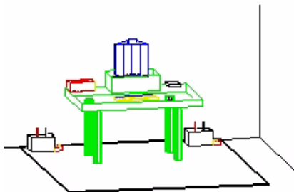
Figure 7-7. Test Instrument & Measurement Setup
