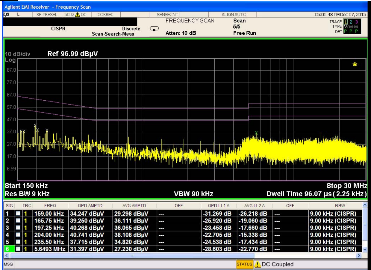
Plot 7-46. Line Conducted Plot with 802.11b (N)
