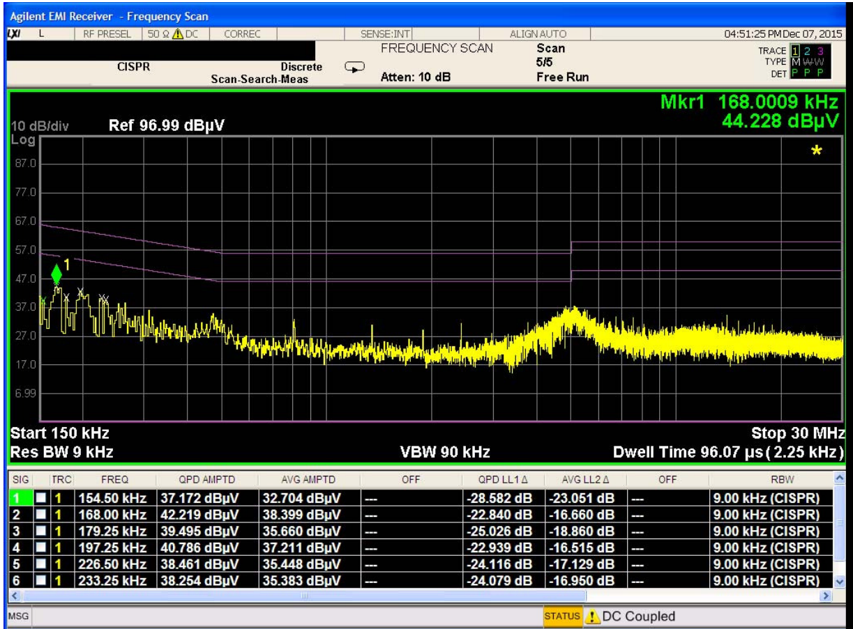
Plot 7-45. Line Conducted Plot with 802.11b (L1)
