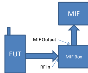
Figure 7-2 MIF Measurement Setup for unlicensed modes
