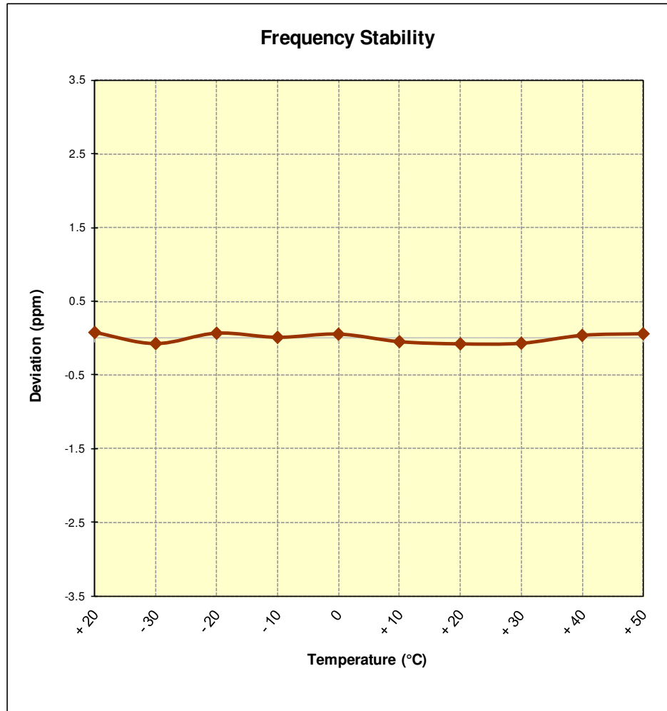
Figure 7-10. Frequency Stability Graph (AWS WCDMA Mode – Ch. 1413)
