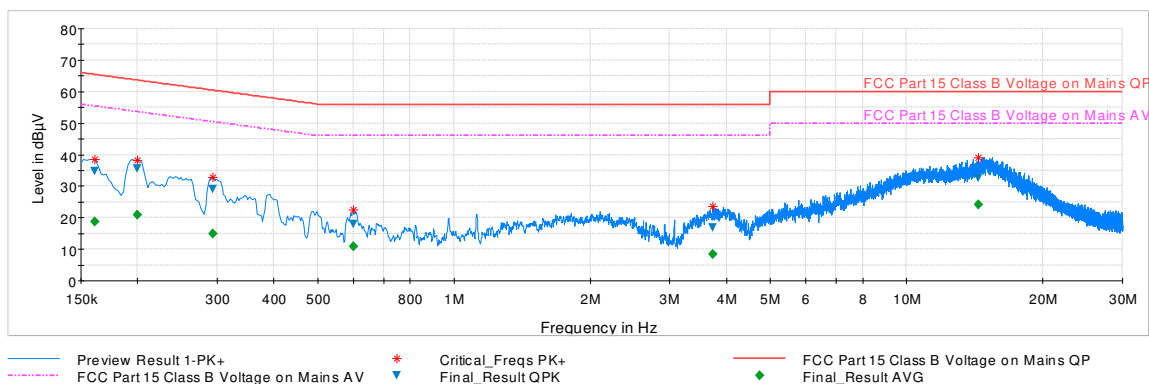
Plot 7-54. Line-Conducted Test Plot (L1)
