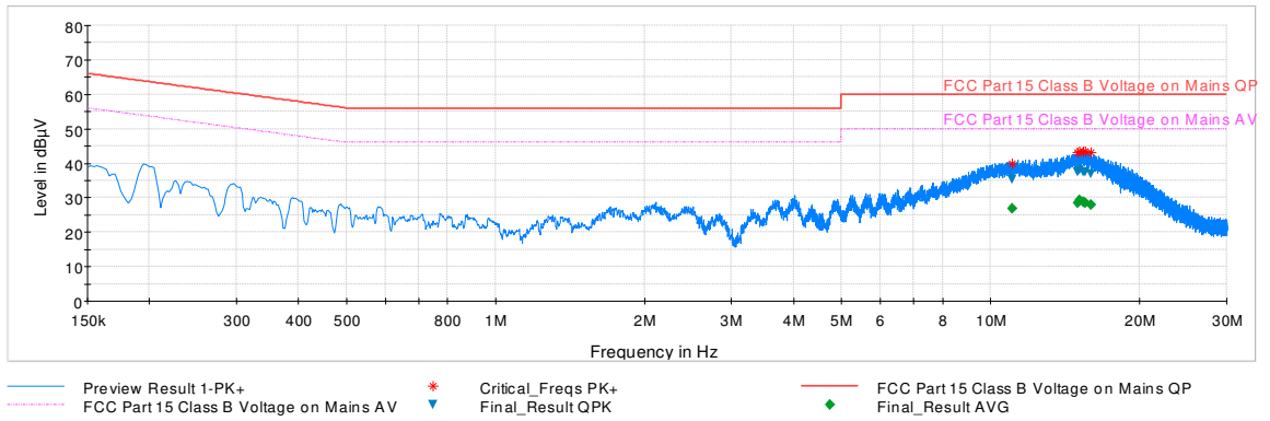
Plot 7-55. Line-Conducted Test Plot (N)
