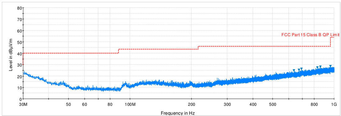
Plot 7-52. Radiated Spurious Plot below 1GHz (Pol. V)
